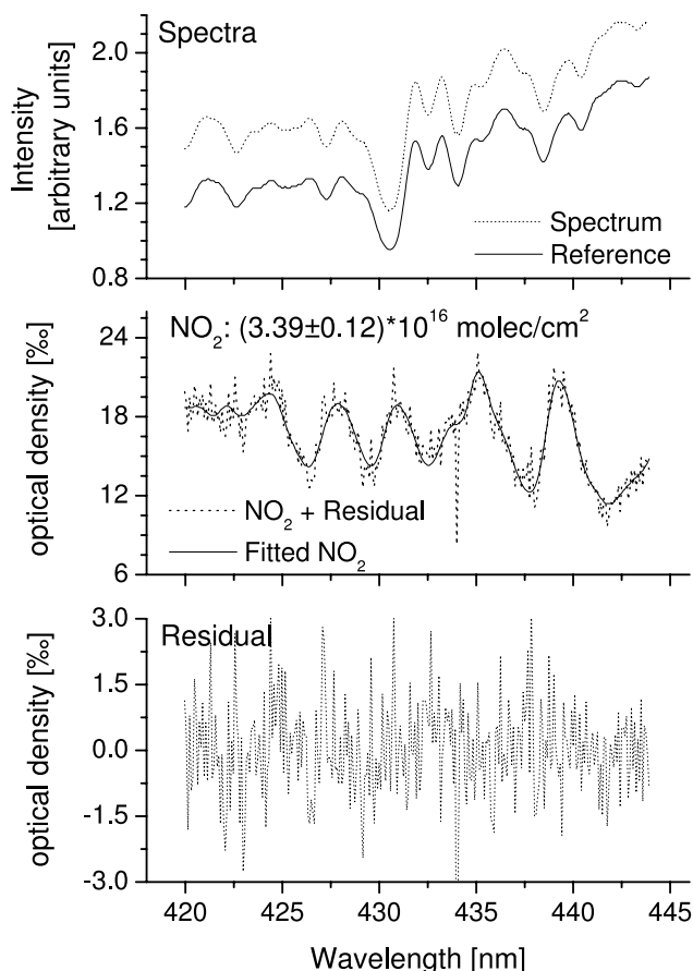
Fig. 3. NO 2 -fit for a Nadir spectrum taken on the flight on 19/02/2003 from Basel to Tozeur at 8:14:30 close to Zürich, the reference was taken about 15 min later in the clean air of the Alps.
