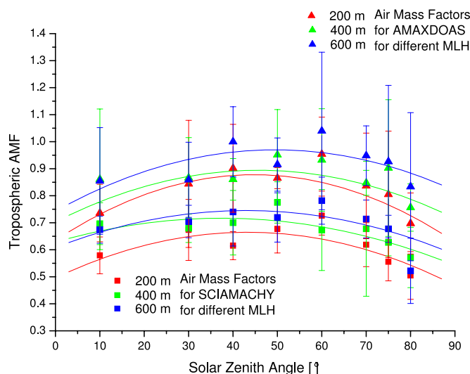
Fig. 5. The AMF for both instruments SCIAMACHY and AMAXDOAS. In general AMAXDOAS is more sensitive to tropospheric pollution than SCIAMACHY. The NO 2 was assumed to be well mixed within the mixing layer and 0 above. Different heights of the ML were assumed and the total aerosol optical thickness was assumed to be constant. The sensitivity decreases slightly from 600 m MLH to 200 m.
