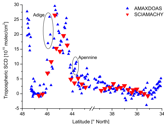
Fig. 10. Slant NO 2 columns measured by SCIAMACHY and AMAXDOAS. In the gaps between two SCIAMACHY Nadir scans no data are shown.
