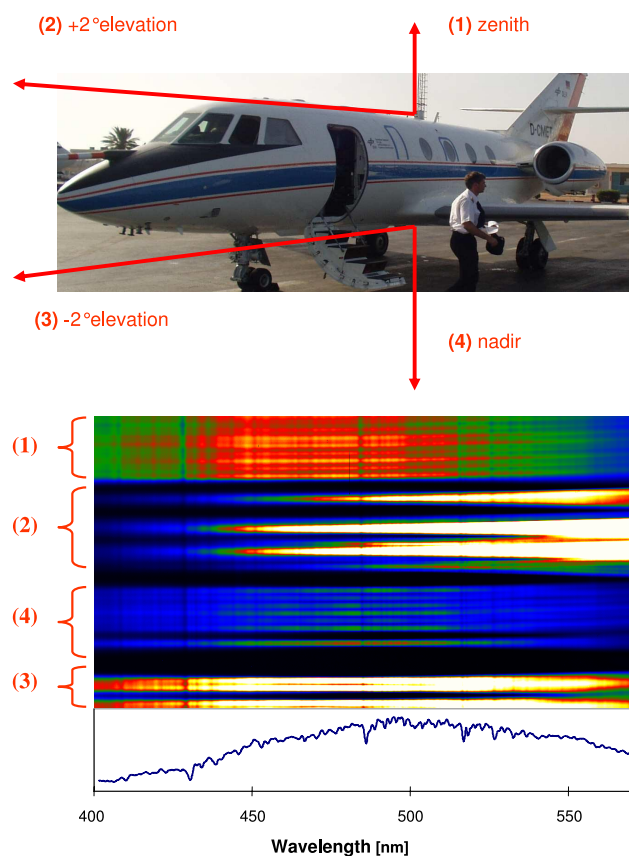
Fig. 2. (a) Upper panel: Pictures of the DLR-Falcon, including a sketch of the used lines of sights. (b) Lower panel: Typical image of vis CCD – the different viewing directions are separated from each other by dark lines. The numbers on the left side belong to the different LOS as marked in Fig. 2a. Usually the direction -2^\circ was the brightest one and therefore only a small area on the chip is used for it.
