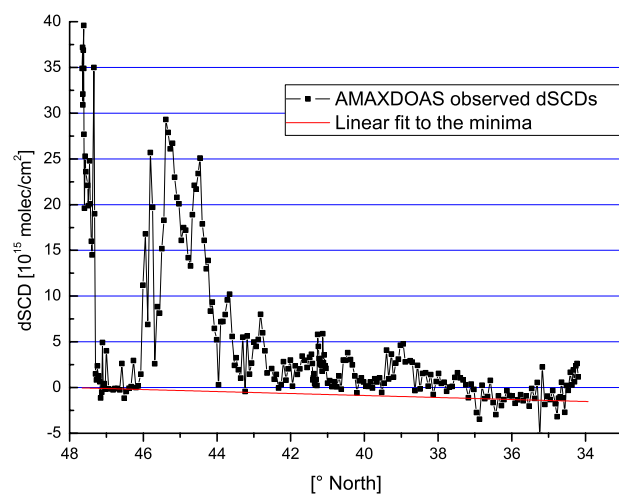
Fig. 4. The observed dSCD from AMAXDOAS and the linear correction (red) for the stratospheric signal. The tropospheric signal was assumed to be negligible in the Alps (47° N) and over the Mediterranean south of Sardegna (36° N).
