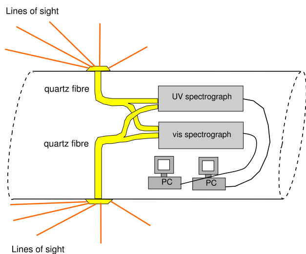
Fig. 1. Sketch of the instrumental setup. Here 2 \times 5 lines of sight are shown. The scattered sunlight is observed using small telescopes and is led to two spectrographs via quartz fibres. Here it is analysed and the spectra are saved on a PC.
