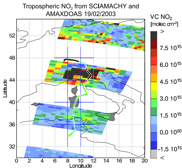
Fig. 9. Tropospheric vertical NO 2 column measured by AMAXDOAS and SCIAMACHY. The AMAXDOAS data were overlaid over SCIAMACHY's pixel in the same scale using very similar colours. Zürich is not covered by SCIAMACHY's pixel on this day.
