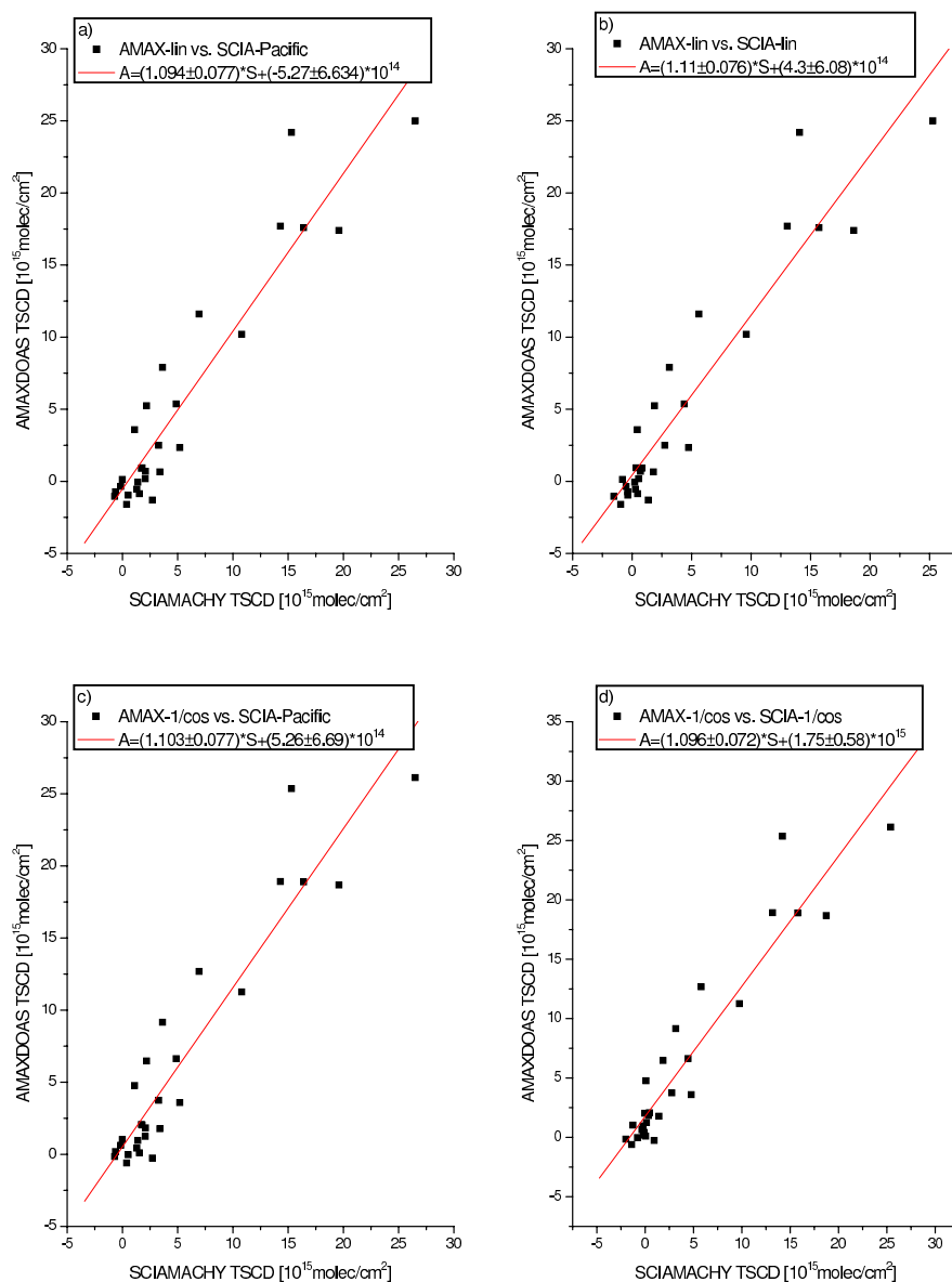
Fig. 11. Correlation between the tropospheric slant column densities measured by SCIAMACHY and AMAXDOAS for different methods of separation between stratospheric and tropospheric absorption. Upper left panel: Reference for SCIAMACHY and linear fit for AMAXDOAS. Upper right panel: For both instruments a linear fit was used. Lower left panel: reference for SCIAMACHY and 1/\cos(SZA) for AMAXDOAS. Lower right panel: 1/\cos(SZA) was used for both.
