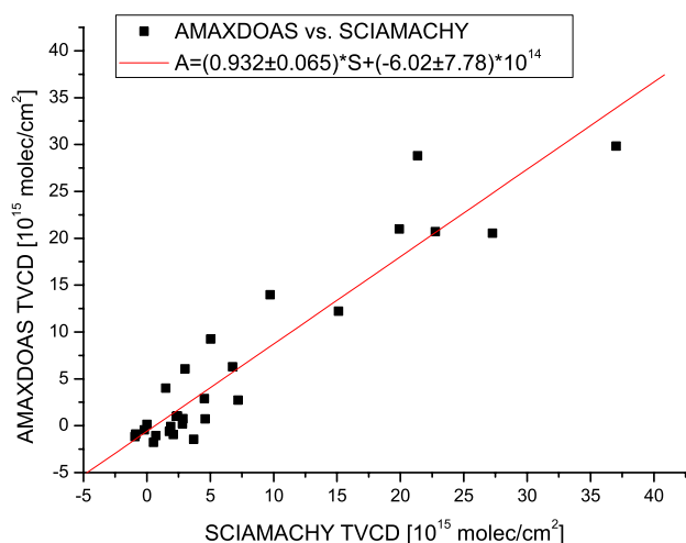
Fig. 12. Correlation of the tropospheric vertical columns. The reference method was used for SCIAMACHY and the linear fit for AMAXDOAS. The AMF was calculated assuming a MLH of 200 m and a total aerosol optical thickness of 0.3.
