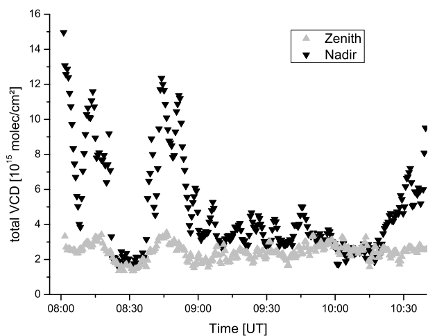
Fig. 7. Time series of the vertical NO 2 columns for AMAXDOAS Nadir and Zenith observations. In Nadir a strong enhancement is observed from 8:40 until 8:55. Here stratospheric AMFs were used, to show the slowly varying stratospheric signal and the influence of tropospheric pollution on the telescope directed to the zenith.
