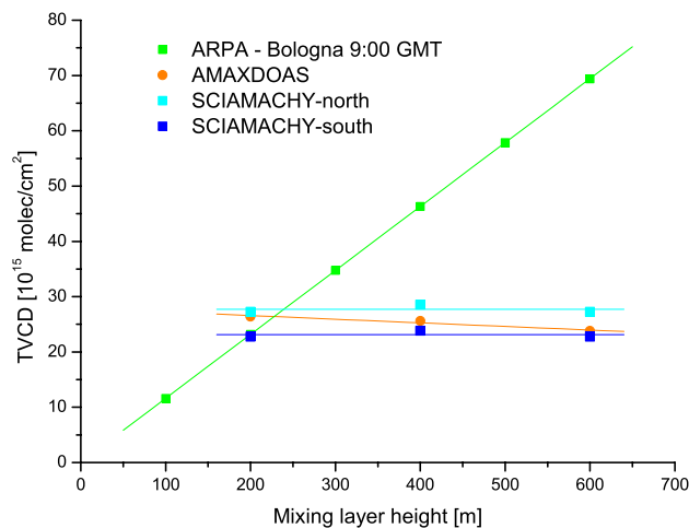
Fig. 8. The tropospheric vertical column calculated for different mixing layer heights. The in situ measurements are shown in green, the AMAXDOAS TSCDs in orange and SCIAMACHY data in blue. As the position of the measurement stations is close to the border between two SCIAMACHY pixels, the data of both pixels are shown here. The southern pixel (dark blue) partly covers the Apennine Mountains.
