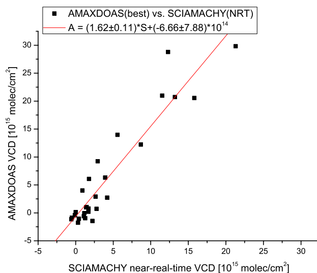
Fig. 13. Correlation between the SCIAMACHY near-real-time data set and the AMAXDOAS data validated with the ground based in situ data.
