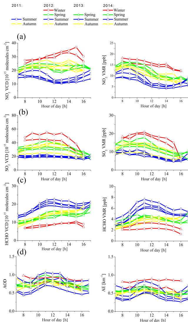
Figure 14. Seasonally averaged diurnal variations of trace gas VCDs and AOD (left panels) and near-surface values (right panels) of NO 2 (a), SO 2 (b), HCHO (c) and aerosols (d) from 2011 to 2014.
