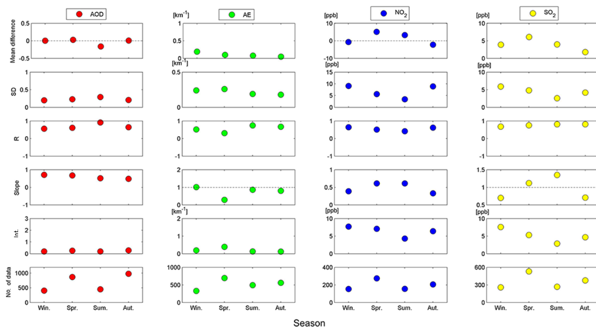
Figure 6. Mean absolute differences and standard deviations as well as correlation coefficients ( R ), slopes and intercepts derived from linear regressions of the AODs, and near-surface AE, \text{NO}_2 and \text{SO}_2 VMRs between MAX-DOAS and independent techniques for different seasons for clear-sky conditions with low aerosol loads. The corresponding number of data points is shown in the bottom panel. Different colours denote AOD (compared with the Taihu AERONET level 1.5 data sets), AE (compared with the nearby visibility meter) and \text{NO}_2 and \text{SO}_2 (compared with the nearby long-path DOAS instrument). For calculations of mean absolute differences, the data derived from independent techniques are subtracted from those derived from the MAX-DOAS instrument. The data derived from the MAX-DOAS instrument are plotted against those derived from independent techniques for linear regressions.
