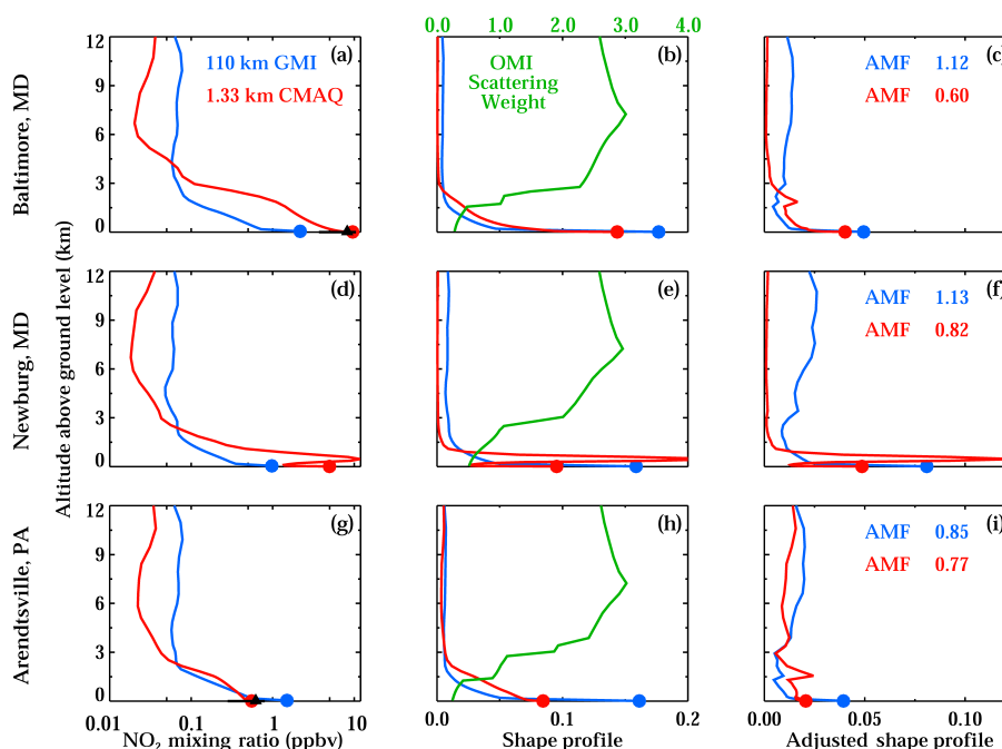
Figure 2. (a, d, g) Mean 14:00 LT June and July 2011 NO 2 mixing ratio as a function of altitude from a GMI ( 1.25^{\circ} \times 1^{\circ} ; \sim 110\text{ km} \times 110\text{ km} ) model simulation and CMAQ ( 1.33\text{ km} \times 1.33\text{ km} ) model simulation for three locations: (a) downtown Baltimore, (d) Morgantown power plant in Newburg, MD, and (g) Arendtsville in rural Pennsylvania. Black triangles with error bars as discussed in the text represent co-located surface observations from the EPA monitoring network. (b, e, h) NO 2 shape profiles (partial NO 2 columns divided by total NO 2 column) as function of altitude for the same time frame and locations; green line denotes co-located OMI scattering weight. (c, f and i) “Adjusted” shape profiles, partial NO 2 columns divided by total NO 2 columns multiplied by OMI scattering weight, as function of altitude for the same time frame and locations.
