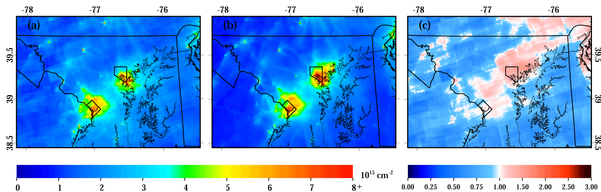
Figure 10. Oversampled tropospheric column NO 2 at 1.33 km in the Baltimore–Washington metropolitan area for June and July 2011 only. (a) OMI_CMAQ_OD. (b) CMAQ NO 2 corresponding to valid overpass times. (c) Ratio between the two plots CMAQ/OMI_CMAQ_OD.
