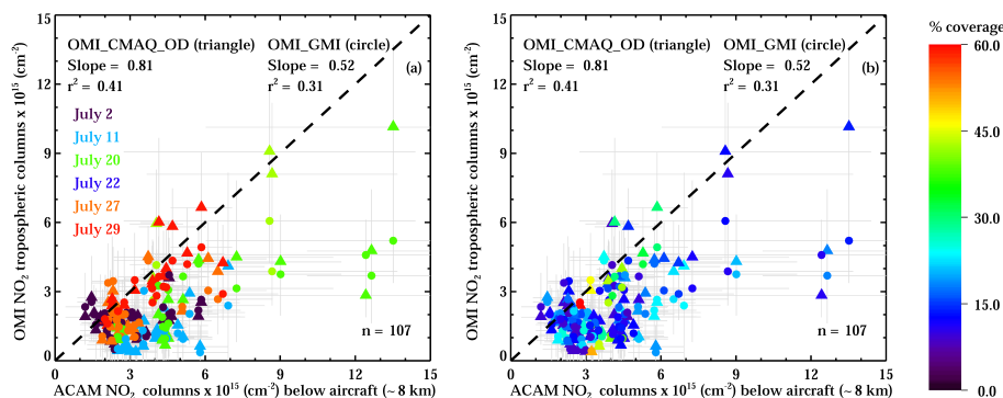
Figure 8. Tropospheric column NO 2 OMI_GMI and OMI_CMAQ_OD vs. co-located spatially and temporally matched ACAM NO 2 column measurements within \pm 1 h of a valid satellite overpass during July 2011. (a) Color-coded based on date. (b) Color-coded based on percent coverage. Error bars on both plots represent \pm 1 SD away from the mean.
