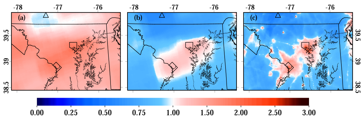
Figure 5. Ratio between the three OMI_CMAQ tropospheric NO 2 retrievals and the operational NASA v3.0 OMI tropospheric NO 2 retrieval for June and July 2008–2012 (2 months \times 5 years; 10 months total). (a) OMI_CMAQ/OMI_GMI. (b) OMI_CMAQ_O/OMI_GMI. (c) OMI_CMAQ_OD/OMI_GMI. In all plots, Arendtsville, PA, is denoted by the triangle in the top left corner.
