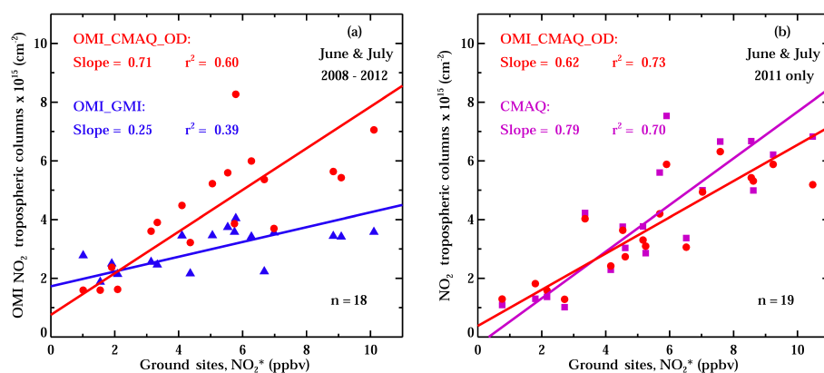
Figure 9. (a) Tropospheric column NO 2 OMI_GMI and OMI_CMAQ_OD vs. co-located ground NO 2 * chemiluminescence measurements within \pm 2 h of a valid satellite overpass during June and July 2008 through 2012; all \sim 300 daily ground monitor values are merged into a mean single value and compared to the satellite mean over the same corresponding time period. (b) Same as (a) but now comparing CMAQ and OMI_CMAQ_OD for June and July 2011 only.
