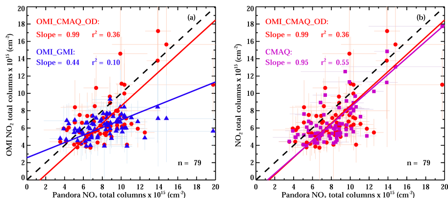
Figure 7. (a) Total column NO 2 OMI_GMI and OMI_CMAQ_OD vs. co-located spatially and temporally Pandora NO 2 total column measurements within \pm 1 h of a valid satellite overpass during July 2011. (b) Same but now showing CMAQ instead of OMI_GMI; the stratospheric vertical column from NASA Level 2 product has been added to CMAQ to ensure a fair comparison. Error bars on both plots represent \pm 1 SD away from the mean.
