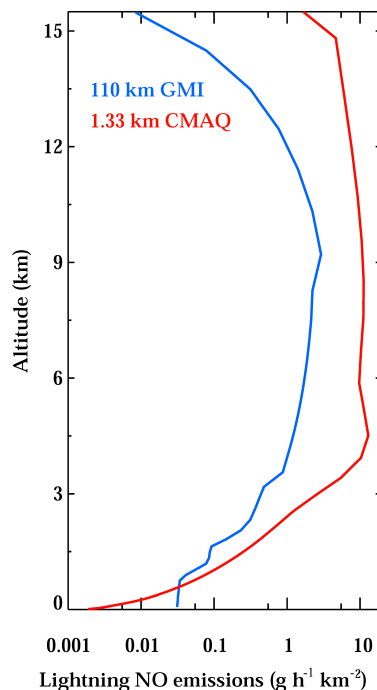
Figure 3. Mean June and July 2011 lightning NO emissions as a function of altitude from the GMI ( 1.25^\circ \times 1^\circ ; \sim 110 \text{ km} \times 110 \text{ km} ) and CMAQ ( 1.33 \text{ km} \times 1.33 \text{ km} ) model simulations.
