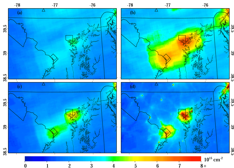
Figure 4. Oversampled OMI NO 2 tropospheric columns at 1.33 km resolution in the Baltimore–Washington metropolitan area for June and July 2008–2012 (2 months \times 5 years; 10 months total). (a) The NASA version 3.0 operational OMI NO 2 product using GMI NO 2 shape profiles (OMI_GMI). (b) OMI NO 2 using CMAQ a priori NO 2 shape profiles (OMI_CMAQ). (c) OMI NO 2 using CMAQ a priori NO 2 shape profiles constrained by observations (OMI_CMAQ_O). (d) OMI NO 2 using CMAQ a priori NO 2 shape profiles constrained by observations and spatial weighting downscaling kernels (OMI_CMAQ_OD). In all plots, Arendtsville, PA, is denoted by the triangle in the top left corner.
