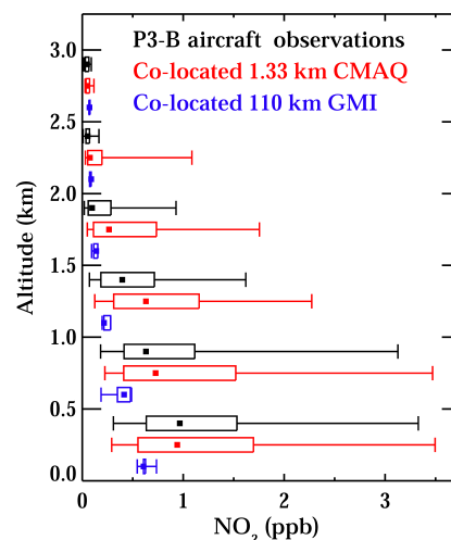
Figure 6. Vertical profiles of NO 2 binned in 500 m intervals (0–0.5, 0.5–1 km, etc.) showing the 5, 25, 50, 75, and 95 percentiles within \pm 2 h of the OMI overpass time. Black: 1 min averaged data from the P3-B aircraft during July 2011 DISCOVER-AQ Maryland. Red: model output from CMAQ matched spatially and temporally to the P3-B measurements at 1 min intervals. Blue: July 2011 monthly mean model output from GMI matched spatially to the P3-B measurements at 1 min intervals. In all cases, the squares indicate the median values.
