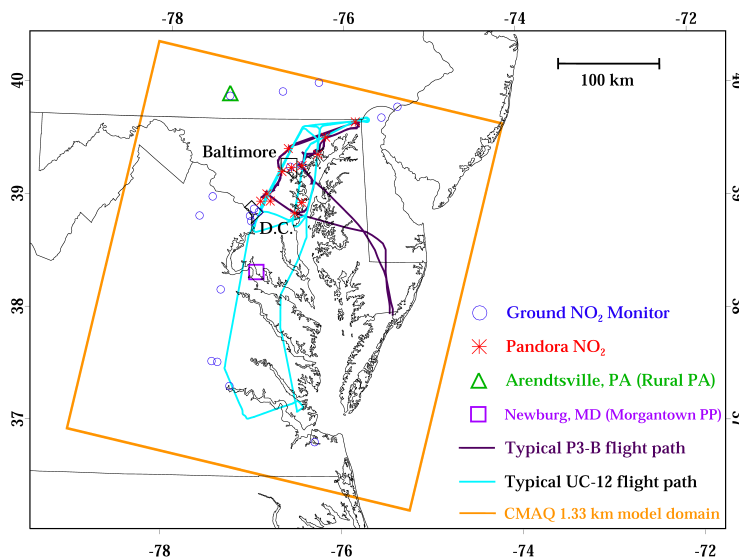
Figure 1. The mid-Atlantic US: the area of interest for this research project. Model domain and observation locations are depicted. There are 18 EPA chemiluminescence NO 2 monitors and 12 Pandora NO 2 measurement sites.
