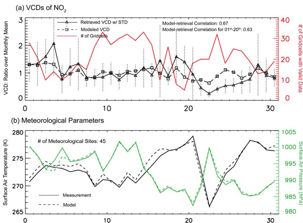
Fig. 10. Daily variations of regional mean VCDs of NO 2 and meteorological parameters in January 2009. (a) Variations of retrieved (OMI_KNMI) and modeled VCDs of NO 2 relative to regional means. Data in a given day are derived as the mean of the ratios of VCDs in gridcells with valid retrievals in that day over monthly mean VCDs in corresponding gridcells. Also shown is the number of gridcells out of the total of 36 over the region in each day that contain valid retrieval data. (b) Variations of measured and modeled daily average surface air temperature and surface air pressure. Meteorological measurements are taken from the global hourly dataset (DS3505) archived in the National Oceanic and Atmospheric Administration (NOAA) National Climatic Data Center (NCDC) ( http://www7.ncdc.noaa.gov/CDO/cdo ; see Lin et al. (2010a)). Daily average values for air temperature (air pressure) are calculated to be means over 3-hourly (6-hourly) data in correspondence to the temporal resolutions of individual model parameters.
