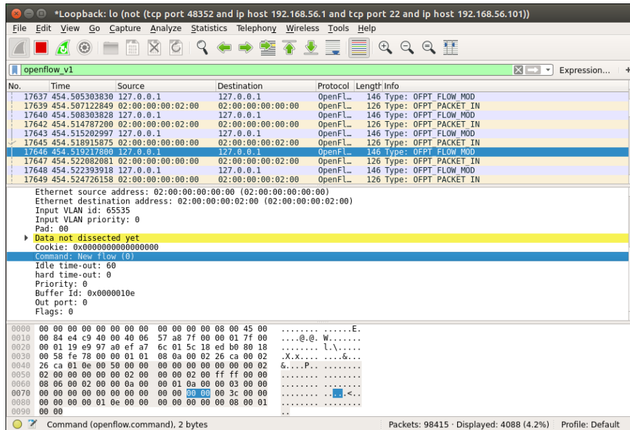
Figure 5.6: Wireshark capturing OpenFlow messages
