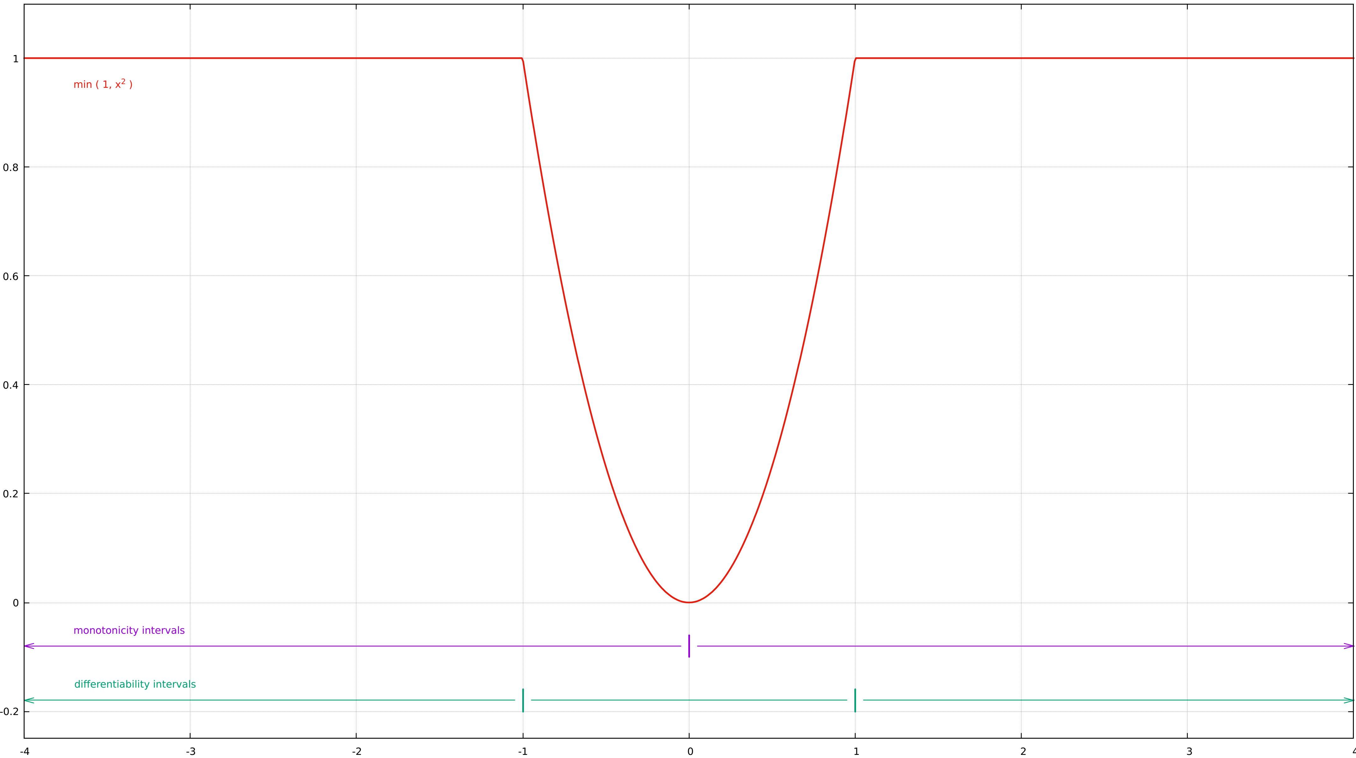
\min ( 1, x^2 ) is piecewise monotonic and piecewise differentiable
