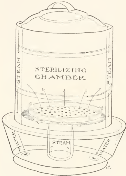
A steam sterilizer.
