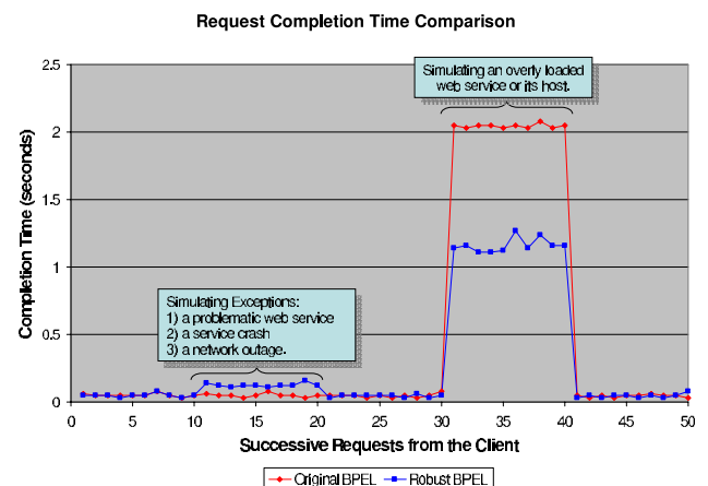
Fig. 15. This chart shows the comparison between the request completion time for the original and the robust BPEL processes.
