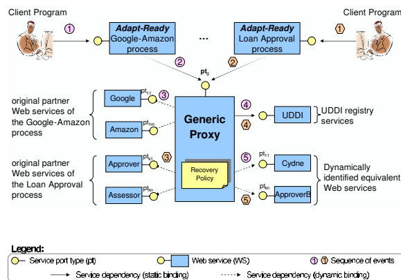
Fig. 16. The interaction between the processes and the generic proxy.
