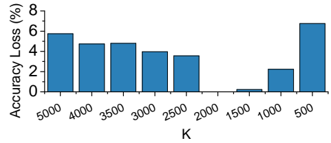
Fig. 16. Machine Translation – Accuracy loss for different values of k using Bag of Words. k =2000 is our baseline.
