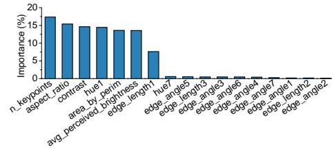
Fig. 13. Image Classification – Accuracy loss if a feature is not used.
