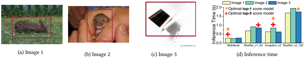
Fig. 1. The inference time (d) of four CNN-based image recognition models when processing images (a) - (c). The target object is highlighted on each image. This example (combined with Table 1) shows that the optimal model ( i.e. the fastest one that gives an accurate output) depends on the success criterion and the input.
