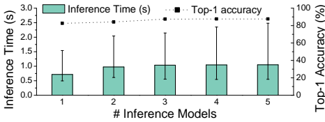
Fig. 18. Overhead and achieved performance when using a different number of DNN models. The range of inference time across testing images is shown using min-max bars.
