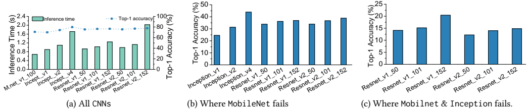
Fig. 7. Image Classification – (a) The top-1 accuracy and inference time of all CNNs we consider. (b) The top-1 accuracy of all CNNs on the images on which MobileNet_v1_100 fails. (c) The top-1 accuracy of all CNNs on the images on which MobileNet_v1_100 and Inception_v4 fails.
