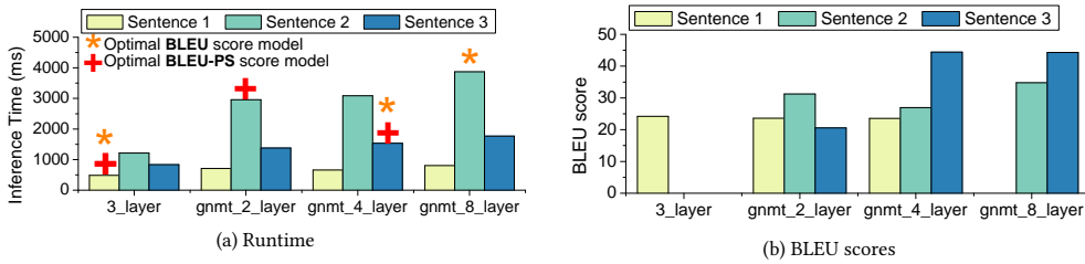
Fig. 2. The inference time, optimal model (a), and BLEU score (b) of three sentences (shown in Table 2). Here the optimal model achieves the highest score for an evaluation criteria. Model names explained in footnote 3.
