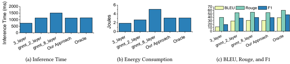
Fig. 10. Machine Translation – Overall performance of our approach against individual models and an Oracle.
