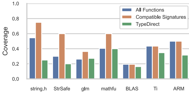
Figure 4: Proportion of each library’s API that we were able to successfully synthesize, across all functions in the library as well as those with compatible type signatures. Results are also shown for TYPEDIRECT [11].
