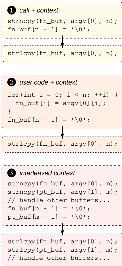
Figure 2: Example of three contexts in which M 3 is able to perform contextual API migrations using only the behavior of the source and target functions.
