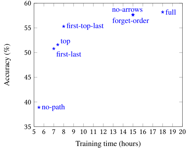
Figure 12. The accuracy of each abstraction method compared to the consumed training time, for the task of variable naming in Java
