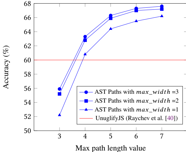
Figure 10. Accuracy results of AST paths with CRFs, for the task of variable naming in JavaScript, for different combination values of max\_length and max\_width (UnuglifyJS is presented here for comparison).
