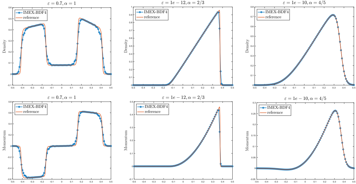
FIGURE 9. Test 4b. Non linear Ruijgrook–Wu model (6.15) with discontinuous initial data (6.19), top column reports the density, bottom column the momentum. Left row \varepsilon = 0.7, \alpha = 1 and final time T = 0.2 , middle row \varepsilon = 10^{-12}, \alpha = 2/3 final time T = 0.5 , right row \varepsilon = 10^{-10}, \alpha = 4/5 , with final time T = 0.5 . The AP-implicit formulation has been used.
