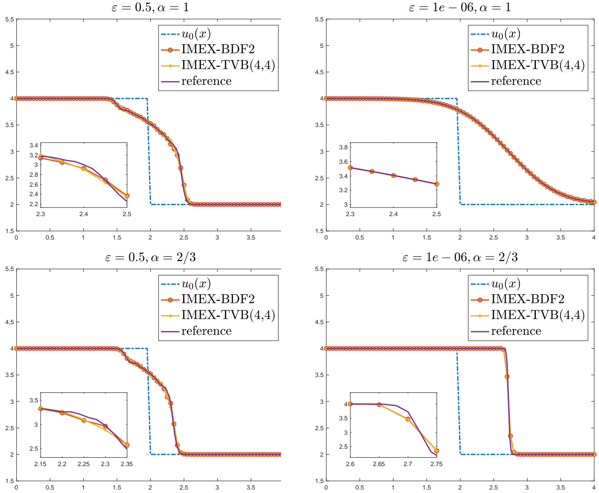
FIGURE 8. Test 4a. Riemann problem for the non linear Ruijgrook–Wu model (6.15) at final time T = 0.25 with AP-explicit methods. Rarefied regime with \varepsilon = 0.5 (left) and limiting behavior for \varepsilon = 10^{-6} (right). Top row \alpha = 1 , bottom row \alpha = 2/3 .
