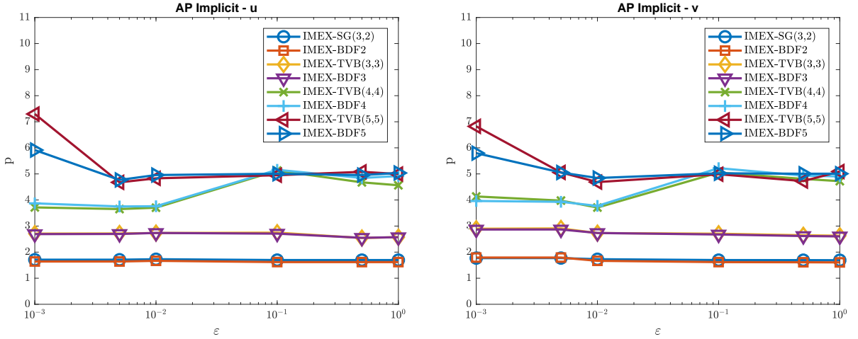
FIGURE 5. Order of convergence of AP-implicit methods in the L_1 -norm using (6.5) for the u variable (left) and the v variable (right).
