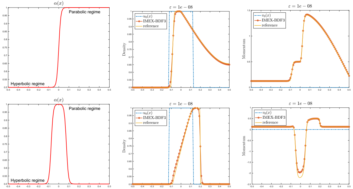
FIGURE 10. Test 4c . Non linear Ruijgrook–Wu model with space dependent \alpha and \varepsilon = 10^{-8} . Left column shows the space variation of the multiscale parameter, whereas the central and right columns depict the evolution of the density u and momentum v from the initial data u_0(x), v_0(x) to final time. Top row accounts a single variation from hyperbolic to parabolic and final time T = 0.05 , whereas second row has two transitions and final time T = 0.1 .
