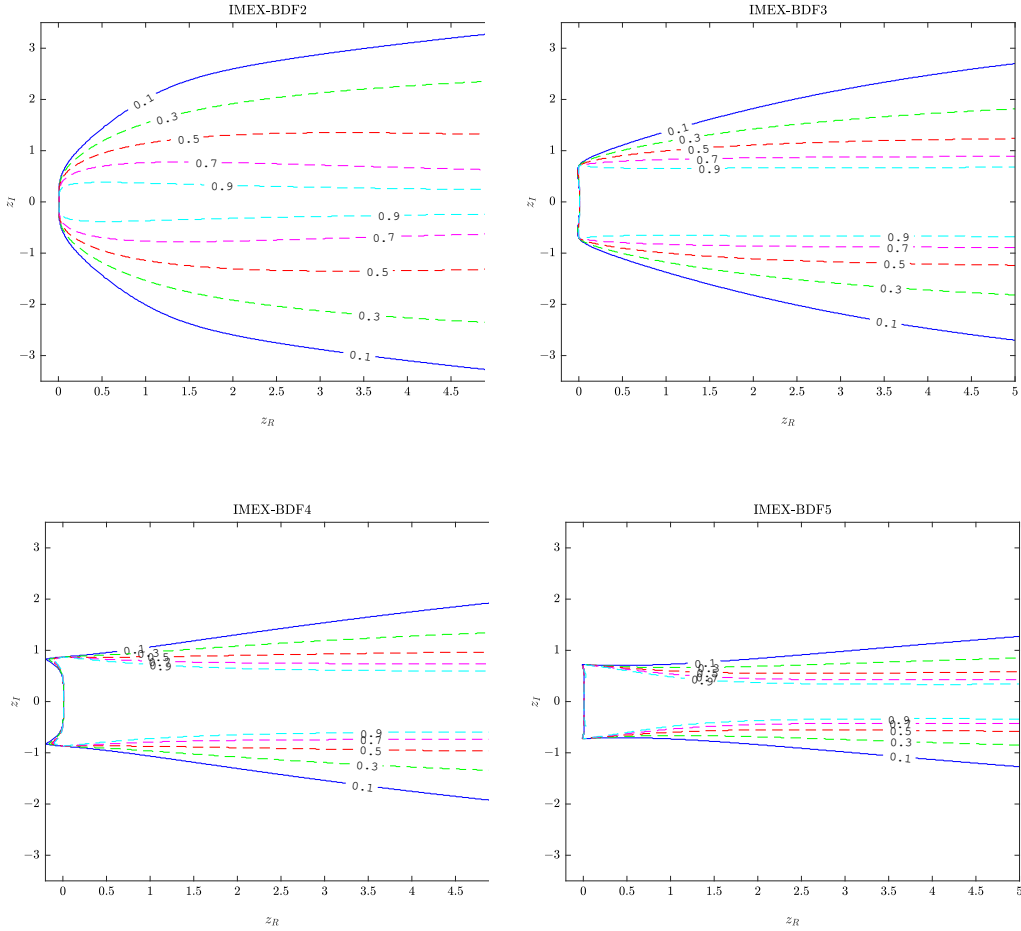
FIGURE 2. AP-explicit methods. Stability regions of IMEX-BDF methods in terms of z_I = i\xi\Delta t/\varepsilon^\alpha and z_R = \Delta t/\varepsilon^{1+\alpha} . The different contour lines correspond to different values of the scaling parameter \varepsilon^\alpha .
