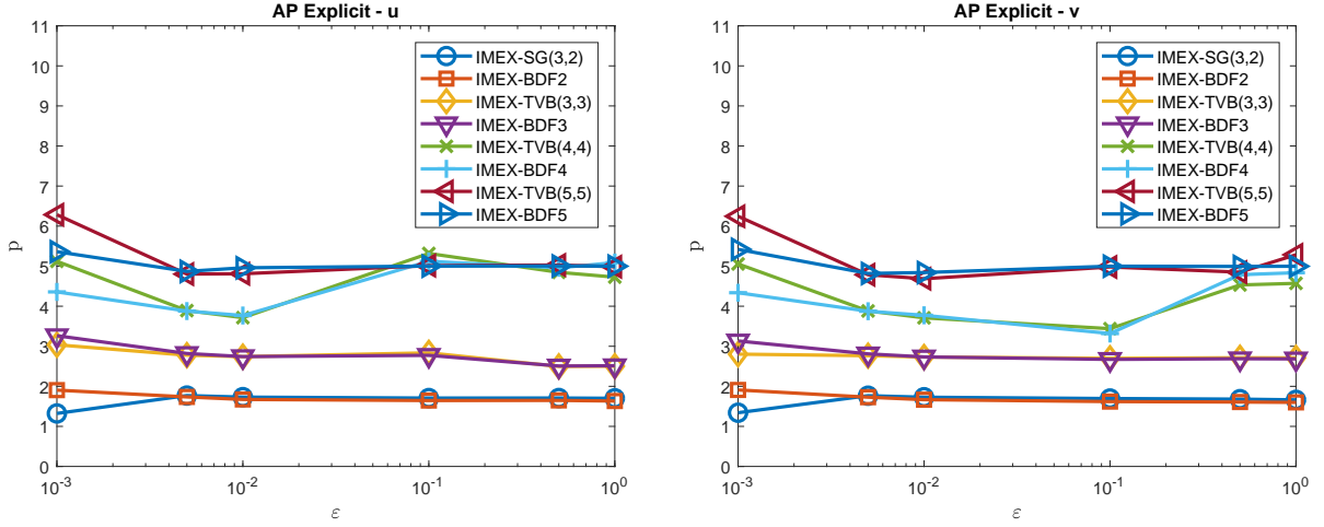
FIGURE 4. Order of convergence of AP-explicit methods in the L_1 -norm using (6.5) for the u variable (left) and the v variable (right).
