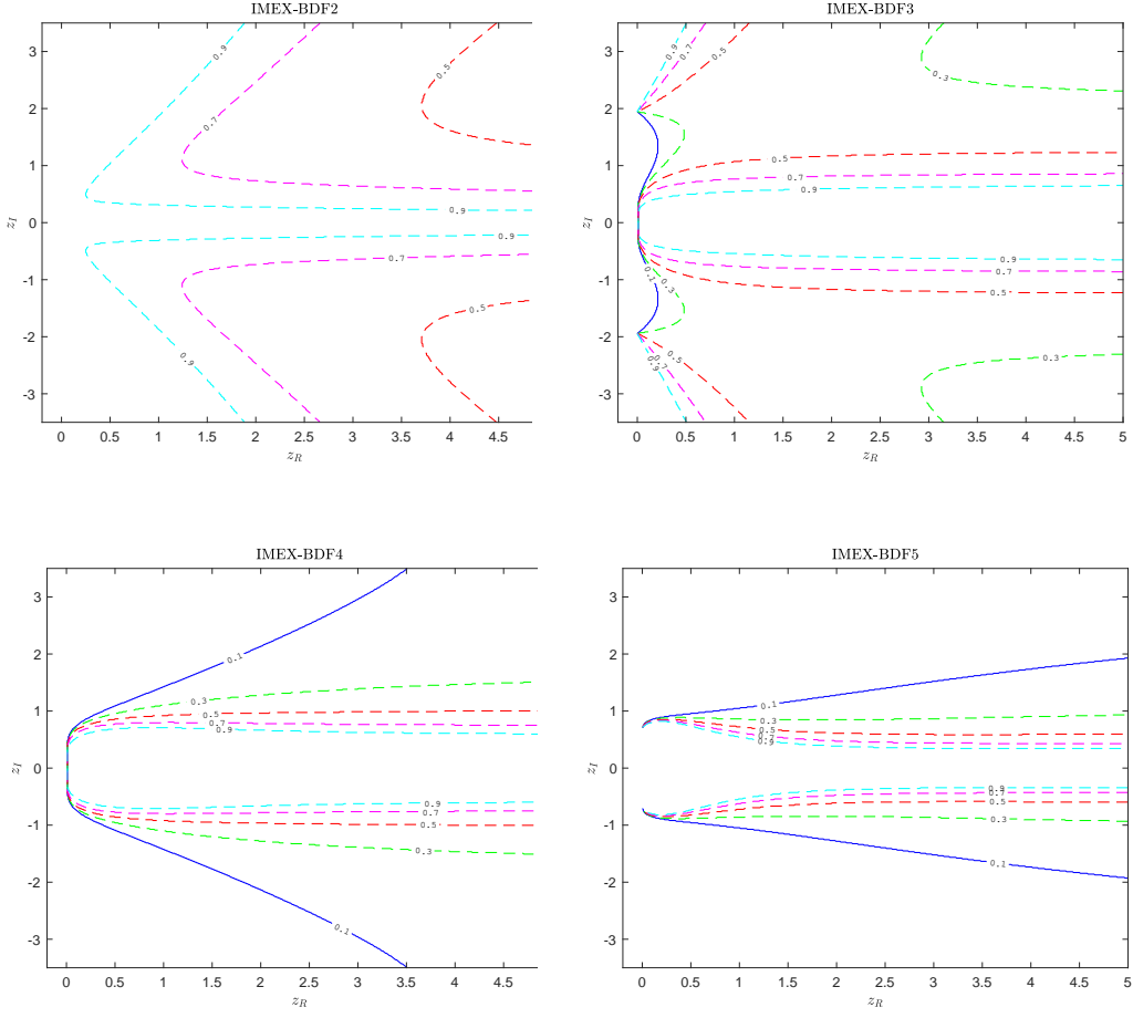
FIGURE 3. AP-implicit methods. Stability regions of IMEX-BDF methods in terms of z_I = i\xi\Delta t/\varepsilon^\alpha and z_R = \Delta t/\varepsilon^{1+\alpha} . The different contour lines correspond to different values of the scaling parameter \varepsilon^\alpha .
