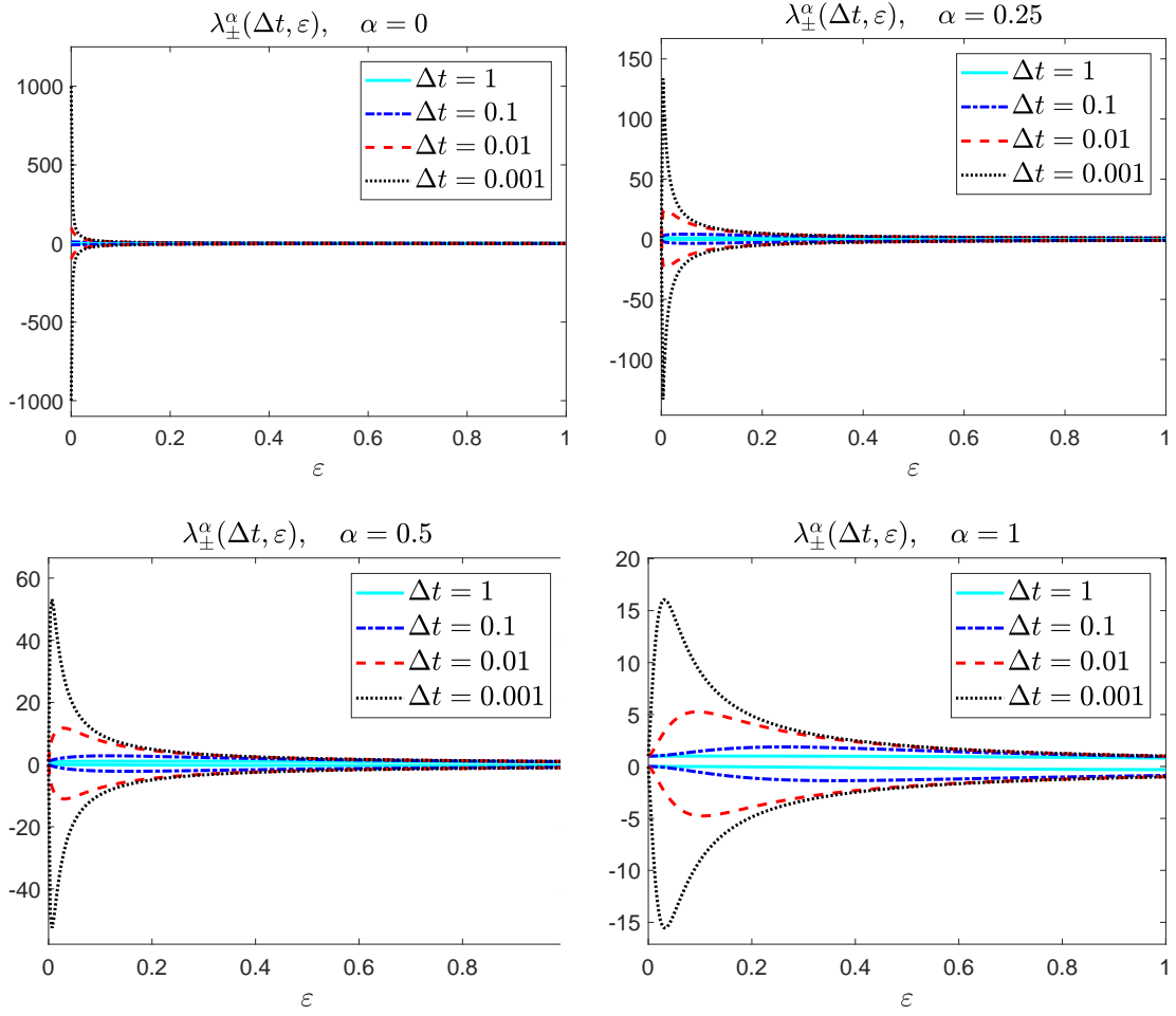
FIGURE 1. Eigenvalues of the modified system (2.7) as a function of \varepsilon for different values of the time step \Delta t and choices of \alpha .
