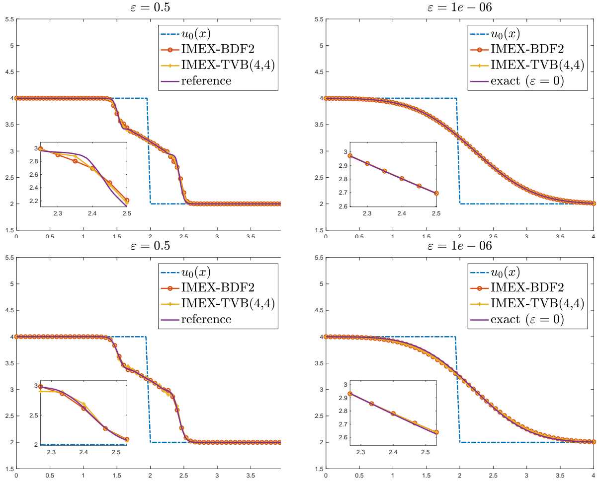
FIGURE 6. Test 2. Riemann problem for linear system with diffusive scaling (6.1) at final time T = 0.25 . Hyperbolic regime with \varepsilon = 0.5 (left) and diffusive regime with \varepsilon = 10^{-6} (right). Top row AP-explicit approach, bottom row AP-implicit approach.
