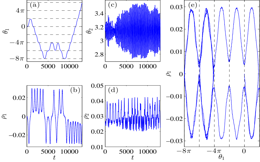
Figure 19. (color online) Same as in Figure 6 but for the full GP model (1.1). Same layout and notation as in Figure 6.
