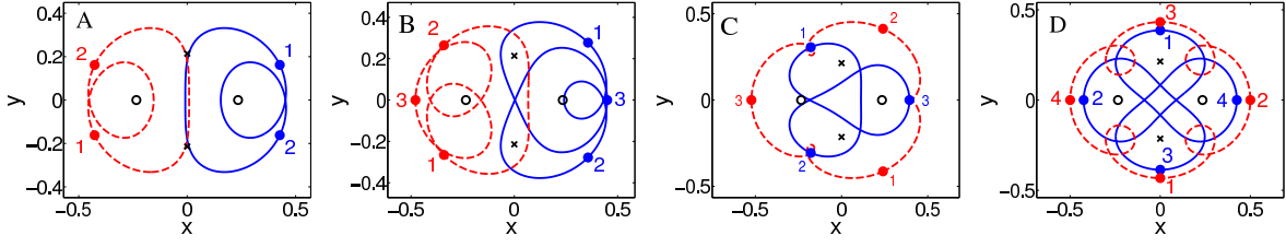
Figure 12. (color online) Periodic vortex paths corresponding with Hamiltonian H = 0.3 , with fewer Poincaré sections than seen in previous figure.
