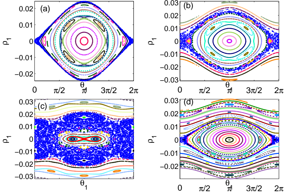
Figure 7. (color online) The Poincaré sections on the hyperplane \theta_2 \equiv \pi \pmod{2\pi} with parameter B = 0.22 in all sections and \epsilon = 0.2 in all but panel (d) where \epsilon = 0.1 . The sections lie on the energy levels (a) H = 0.2246 , (b) H = 0.23 , (c) H = 0.3 , and (d) H = 0.23 . The value of H restricts the allowable values of \rho_1 , which is easily seen in all panels but (c).
