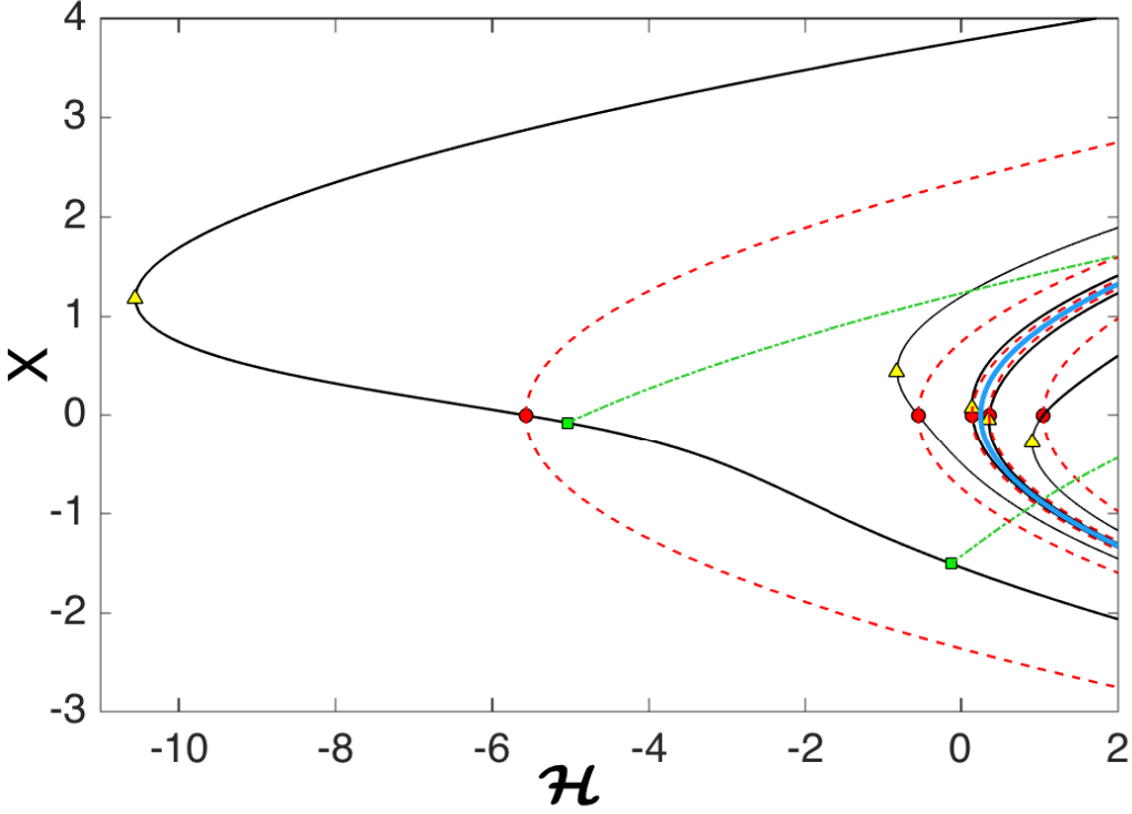
Figure 8. (color online) A partial bifurcation diagram for map (4.8). It shows the separatrix curve \mathcal{S} (light blue), fixed point branches (black line), type-1 period-two points (green dash-dot, real parts only), type-2 period-two points (red dashed), saddle node bifurcations (yellow triangles), type-1 period-doubling points (green squares), and type-2 period-doubling points (red circles).
