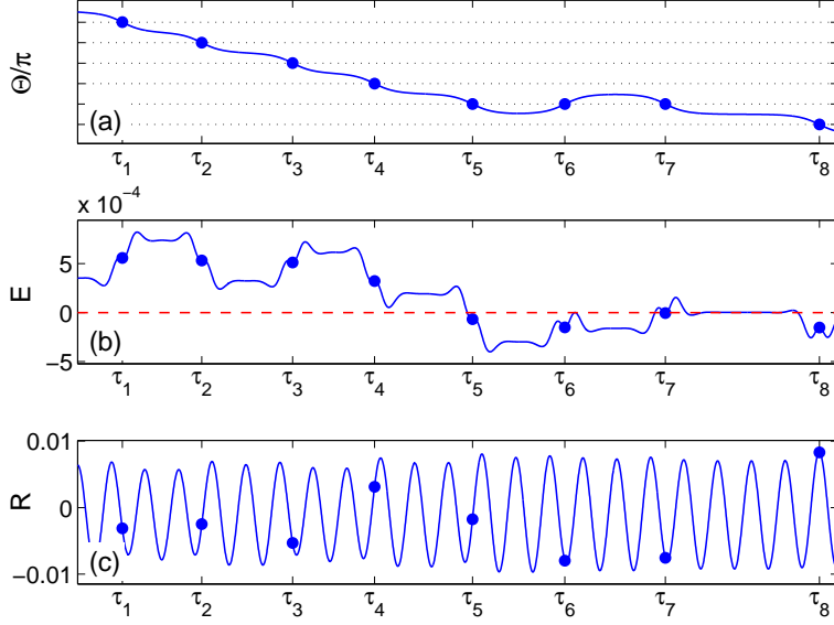
Figure 3. (color online) Figure used in constructing the iterated map. (a) \Theta(\tau) with horizontal dashed lines at \Theta = \pi \pmod{2\pi} , the minima of the potential V(\Theta) = \cos \Theta - 1 . This defines a sequence of times \tau_j (see filled [blue] circles in all panels) at which \Theta(\tau_j) reaches these minima. (b) The energy E(\tau) in the pendulum like component. (c) The evolution of the oscillatory variable R(\tau) .
