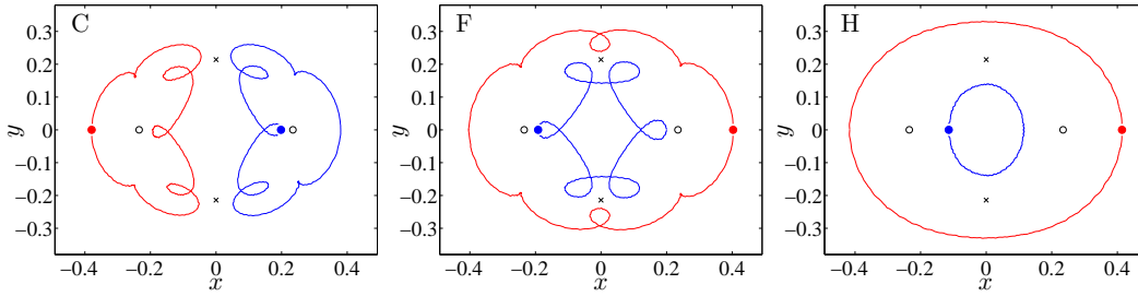
Figure 17. (color online) Same as in Figure 17 for the respective panels of Figure 11 and the bottom panel of Figure 9. Namely, for an energy of H = 0.228 .
