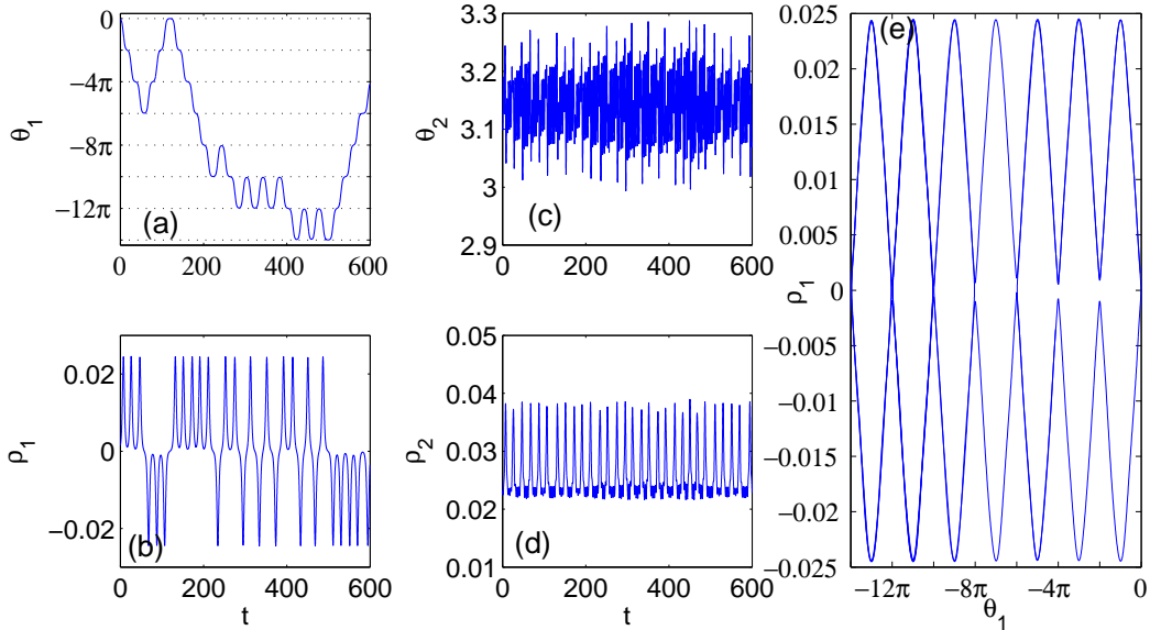
Figure 6. (color online) Numerical solution of initial value problem near the guiding center orbit. (a)-(d), evolution of the components of the solution, (e) phase portrait projected to (\theta_1, \rho_1) coordinates.
