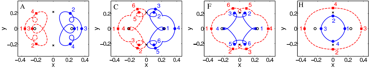
Figure 11. (color online) The solutions with initial condition \rho_2^+ . Only those that intersect the Poincaré section an even number of times are shown.
