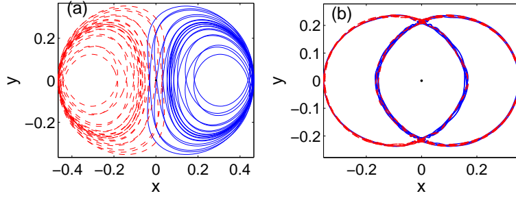
Figure 5. (color online) The reconstructed particle trajectories from (a) the near-separatrix orbit, and (b) the near-guiding center.
