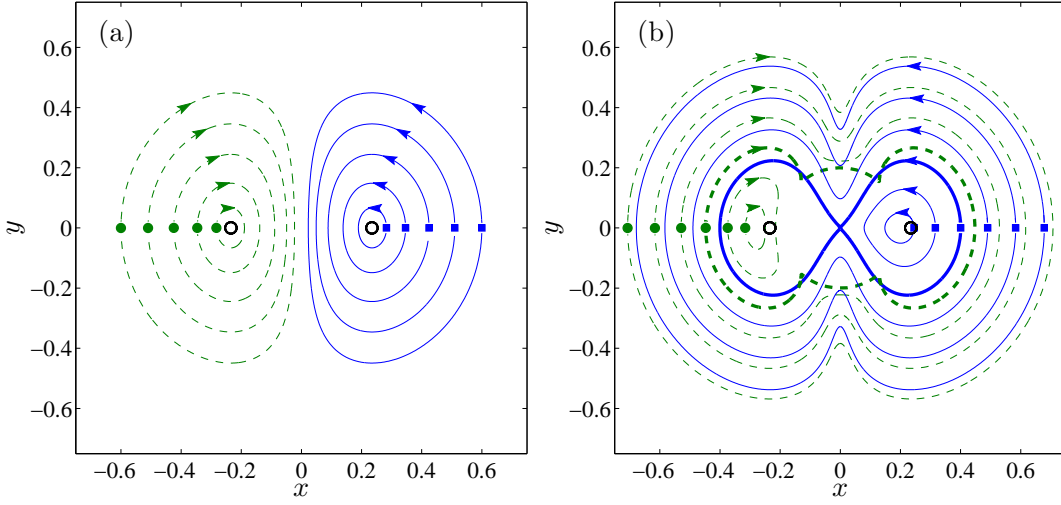
Figure 2. (color online) Typical orbits for two interacting vortices in an isotropic ( \epsilon = 0 ) BEC. The solid (blue) line corresponds to the orbit of one vortex and the dashed (green) line to the orbit of the other vortex. Matching orbits for each pair corresponds to the closest initial conditions (filled squares and circles) pairs from the origin. (a) Closed orbits of two vortices when B = 0.22 and \rho_1 = 0 . At t = 0 , the solutions start on the x -axis at maximal distance apart (see filled squares and circles). They rotate about their centers in opposing directions (see arrows indicating the direction of the orbits), nearly collide and then move off again. (b) “Closed orbits” of the system with \rho_1 = 0.01 , which are closed when viewed in an appropriate rotating reference frame. The orbits depicted with the thick lines corresponds to the the separatrix in Figure 1b. The solutions outside the separatrix cross the line x = 0 without colliding. The equilibrium positions (2.3) are depicted by the black empty circles.
