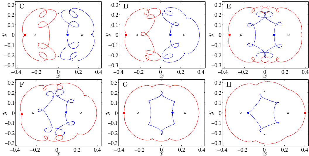
Figure 16. (color online) Periodic orbits of the full GP model (1.1) with an anisotropic potential (6.2) with \epsilon = 0.2 . The initial conditions were found by using the initial conditions corresponding to the periodic orbits of the reduced ODE system (2.1) as seeds for a local search in initial condition space (see text for details). The different panels are labelled using the same notation as the respective panels in Figure 10 and the top panel of Figure 9. Namely, for an energy of H = 0.228 .
