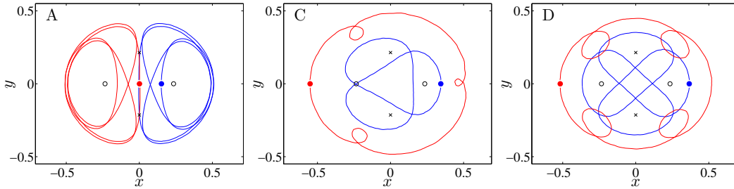
Figure 18. (color online) Same as in Figure 18 for the respective panels of Figure 12. Namely, for an energy of H = 0.3 .
