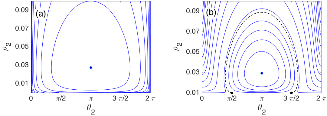
Figure 1. (color online) Phase plane of reduced system (3.1) with B = 0.22 with (a) \rho_1 = 0 and (b) \rho_1 = 0.01 .
