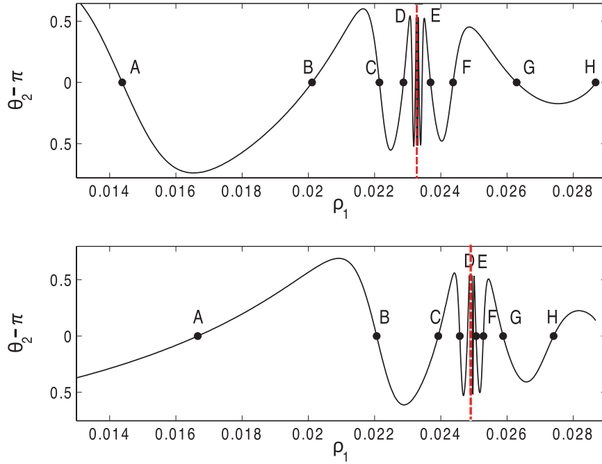
Figure 9. (color online) The value of \theta_2(T) - \pi when the solution to system (2.5) is on the Poincaré section \theta_1 = \pi . As described in the text, zeros of this function determine symmetric periodic orbits of the system. Top: initial condition \rho_2(0) = \rho_2^- . Bottom: initial condition \rho_2(0) = \rho_2^+ . This curve is defined for -\rho_1^* < \rho_1 < \rho_1^* , but is symmetric about \rho_1 = 0 , and has no zeros on the interval (0, 0.014) .
