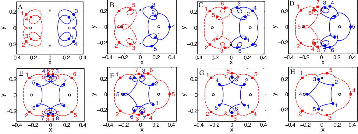
Figure 10. (color online) Periodic orbits of system (2.5) with H^* = 0.228 and the larger value of \rho_2 chosen as the initial condition. Note the \rho_1 -interval on which this is defined is about [-0.029, 0.029] , but the curve is symmetric about zero, and has no roots between \rho_1 = 0 and the intersections marked ‘A’ (see Figure 9). The points depicted by the black empty circles and crosses correspond to the two pairs of vortex dipole steady state solutions of equation (2.3).
