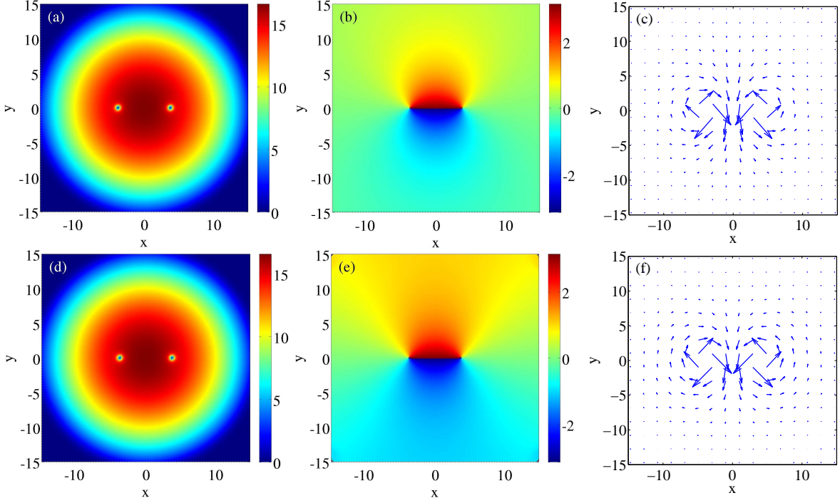
Figure 13. (color online) Steady state dipole configurations. The top row depicts (a) density, (b) phase, and (c) fluid velocity for a vortex dipole seeded, using the approximate solution (6.3), at the steady state position (2.3) on an isotropic BEC. Similarly, the bottom row depicts the actual steady state solution for the stationary vortex dipole using a Newton-type fixed point iteration method. The fluid velocity corresponds to the gradient of the phase.
