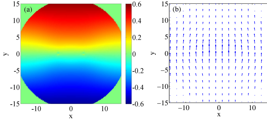
Figure 15. (color online) Difference between the steady state dipole vortex configuration seeded using equation (6.3) (see top row of panels of Figure 13) and the numerically exact solution (see bottom row of panels of Figure 13). Panels (a) and (b) depict, respectively, the difference between the phases and the fluid velocities.
