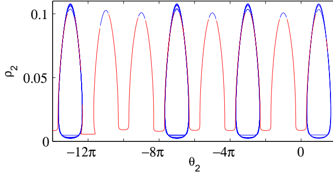
Figure 4. (color online) The (\theta_2, \rho_2) component of the motion near the separatrix of Figure 1. The solution is plotted in red when the instantaneous energy H_0(\theta_2, \rho_1, \rho_2) lies below the separatrix value and in blue when it lies above.
