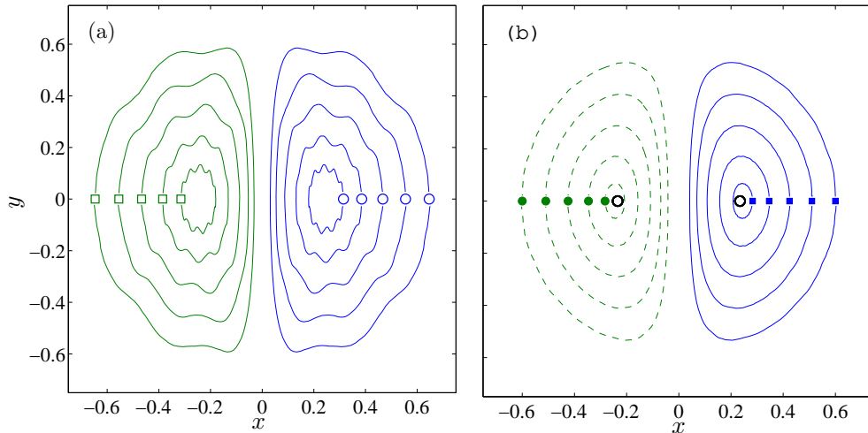
Figure 14. (color online) (a) Orbits generated by the full GP dynamics of a vortex dipole seeded in the BEC using equation (6.3). The orbits are similar to the ones obtained using the ODE reduction as in Figure 2a. However, notice the spurious “wiggles” present in all GP dynamics. (b) Corresponding orbits after subtracting the linear momenta of the initial configuration (6.3). Note that the wiggles are no longer present.
