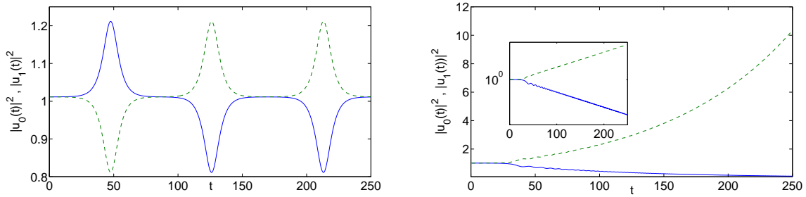
Figure 6: The left panel shows the evolution of the unstable in-phase solution for \gamma = 0 . The amplitude of the central-most two nodes is shown as a function of time. The symmetry-breaking results from the amplification of a noise in the initial data and manifests the instability via a (nearly) periodic recurrence between symmetry-restored and symmetry-broken phases. The right panel shows the same instability for \gamma = 0.5 . The instability leads to an amplification of the gained site amplitude and a decay of the damped site amplitude.
