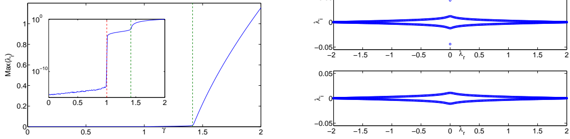
Figure 3: The left panel shows the dependence of the maximal imaginary part \lambda_i of the eigenvalues \lambda = \lambda_r + i\lambda_i versus \gamma for N = 1 . While this is shown in a linear scale with the green dashed line denoting the bifurcation point \tilde{\gamma}_1 = \sqrt{2} , the inset in a semi-logarithmic scale demonstrates the finite-size instability emerging at \gamma = 1 , which is denoted by the red dashed line. The right panel shows the spectrum of the linear PT-dNLS equation (34) for \gamma = 1.43 (top) and \gamma = 1.4 (bottom).
