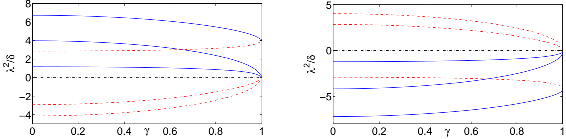
Figure 7: Stability analysis results for the case of N = 2 . The left panel depicts the ++++ solution (which has three real eigenvalue pairs) by solid (blue) lines, as well as the + - - + solution (which has two imaginary and one real pair) by dashed (red) lines. The right panel depicts the + - + - solution (which has three imaginary eigenvalue pairs) by solid (blue) lines, as well as the ++ -- solution (which has two real pairs and one imaginary) by dashed (red) lines. Each pair of these configurations collides and disappears at \gamma = 1 .
