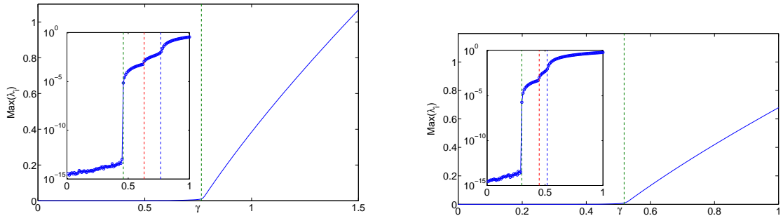
Figure 4: The case of N = 2 (left panel) and N = 3 (right panel) for a finite lattice of 800 sites. The panels are similar to the left panel of Fig. 3, but feature two weak instabilities due to finite size effects (green and red dashed line), in addition to the strong instability at \tilde{\gamma}_N (blue dashed line).
