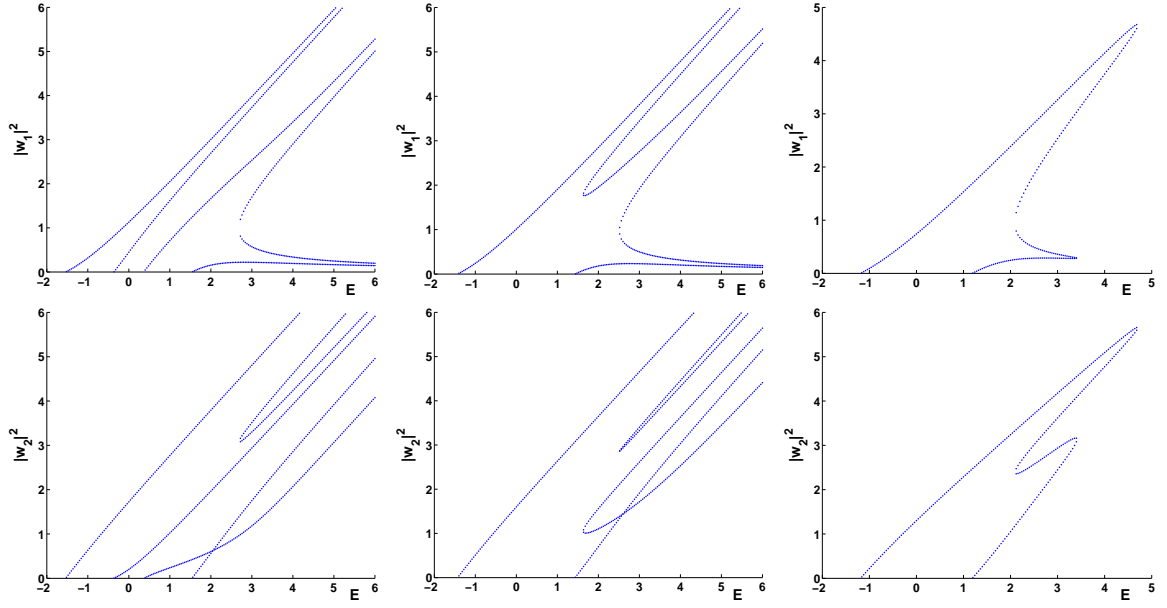
Figure 1: Nonlinear stationary states for N = 2 and for \gamma = 0.5 (left), \gamma = 0.75 (middle), and \gamma = 1.1 (right). The top and bottom rows show components |w_1|^2 and |w_2|^2 respectively.
