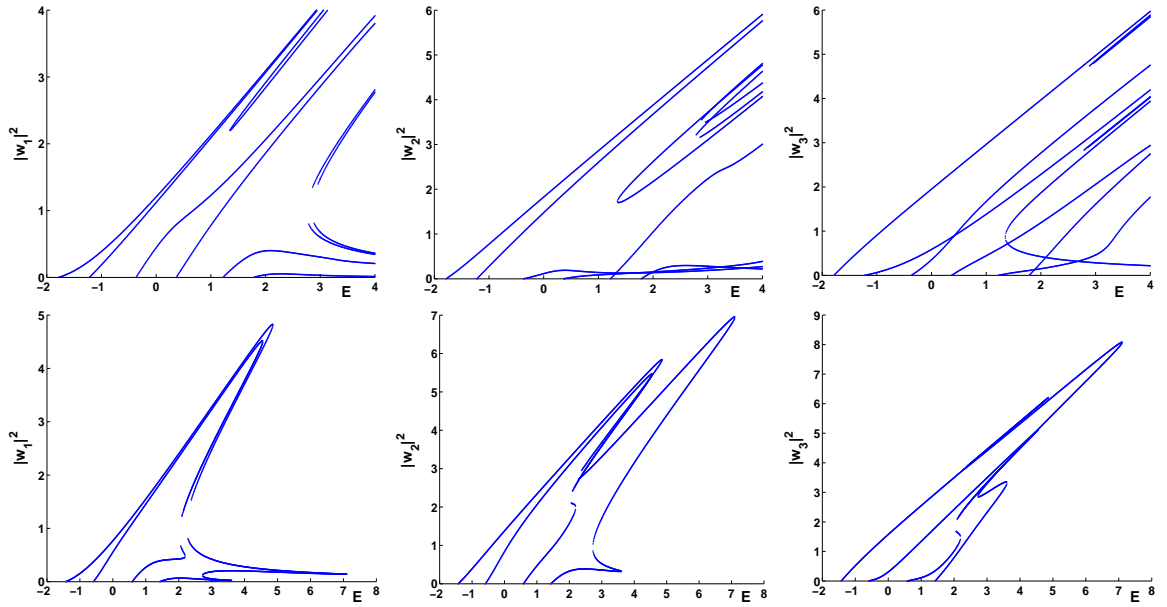
Figure 2: Nonlinear stationary states for N = 3 , and for \gamma = 0.25 (top) and \gamma = 1.1 (bottom). The left, middle, and right columns show components |w_1|^2 , |w_2|^2 , and |w_3|^2 respectively.
