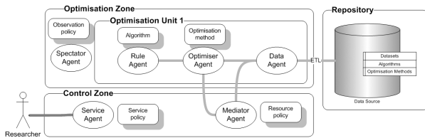
Figure 1. F-TRADE 3.0 architecture
