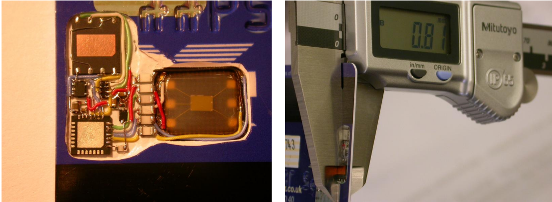
Figure 3: Passive monitoring card containing real EMV chip, with monitoring microcontroller and flash storage
