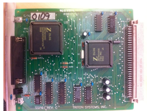
(c) CPU board from Triton ATM
