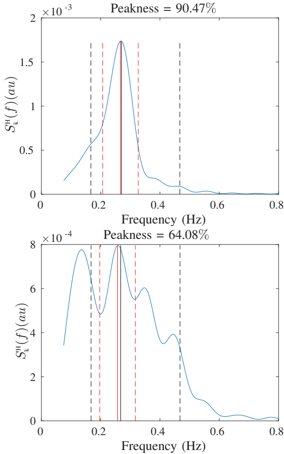
Fig. 4. Differences between spectra that satisfy the peakness condition and spectra that do not. Red lines illustrate the limits of the integrating interval of the numerator in P_{jk}^H with the solid line marking the f_n^H(k) value. Black dashed lines illustrate the reference interval \Omega_R^H(k) , with the solid line representing the previous estimated respiratory rate F_R^H(k-1) .
