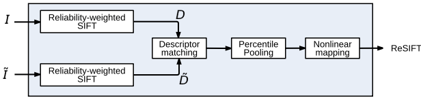
Fig. 2. ReSIFT pipeline
