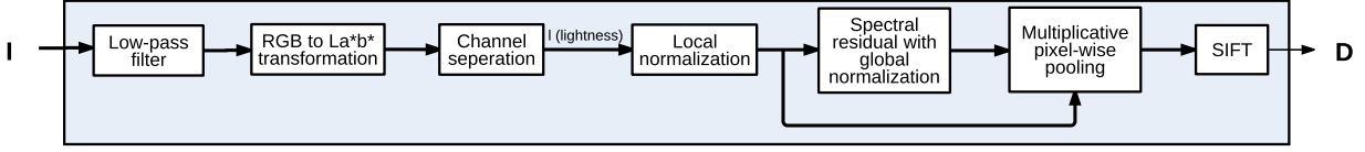
Fig. 1. Reliability-weighted SIFT descriptor extraction
