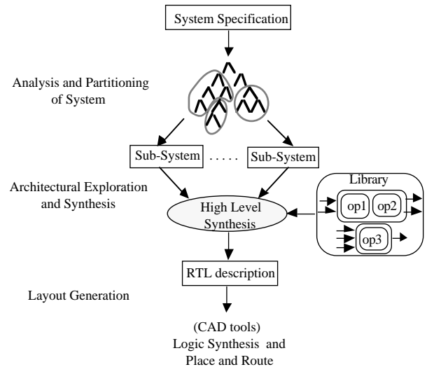
Figure 1: Design-flow
