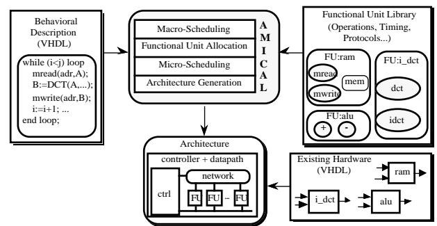
Figure 4: AMICAL design-flow
