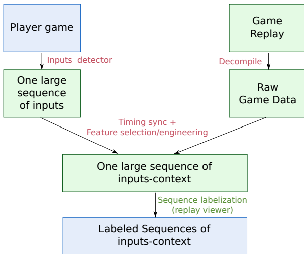
Fig. 3: Data augmentation (expert intervention in blue)
