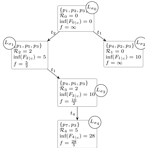
Figure 3 State Graph of cTPN of Fig. 1 using greedy algorithm
