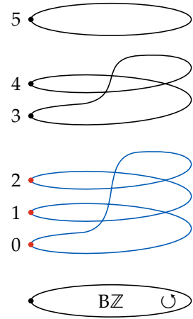
FIGURE 5.2: A \mathbb{Z} -set with three orbits and one fixed point.
