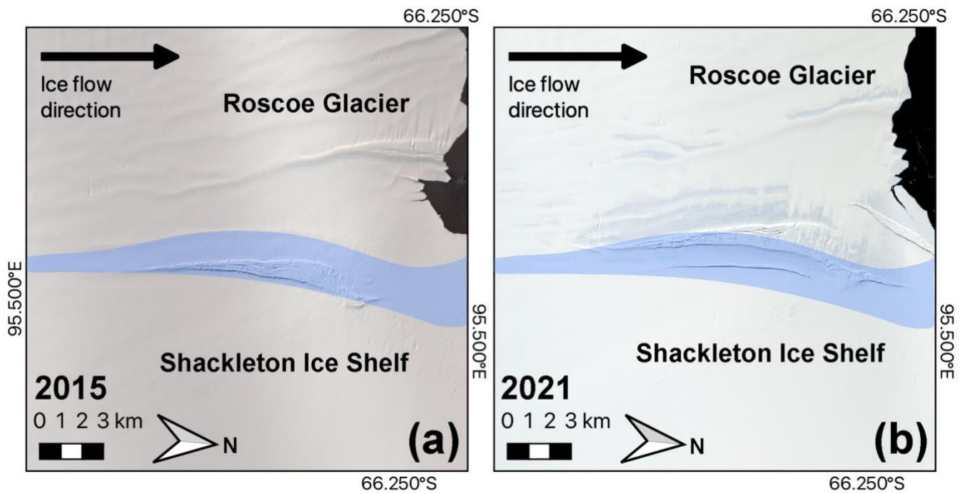
665 Figure 5: Rift opening in the vicinity of the shear margin between the Shackleton Ice Shelf and Roscoe Glacier (location marked in blue) between (a) 2015 (Background: Landsat 8 OLI acquired 14th March 2015 and (b) 2021 (Sentinel 2B acquired 13 th February 2021).
