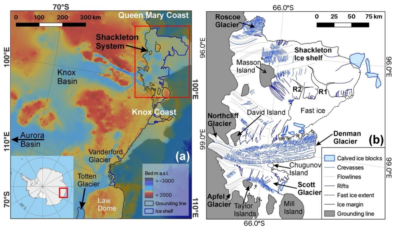
Figure 1: (a) Area of focus in the regional context of the Aurora and Wilkes subglacial basins, location shown in inset (Background: BedMachine V2 (Morlighem et al., 2020)). (b) The Shackleton system overview in February 2021 with the two main rift systems on Shackleton Ice Shelf labelled R1 and R2. All features mapped from Sentinel 2A and 2B imagery acquired 05 th – 27 th February 2021.
