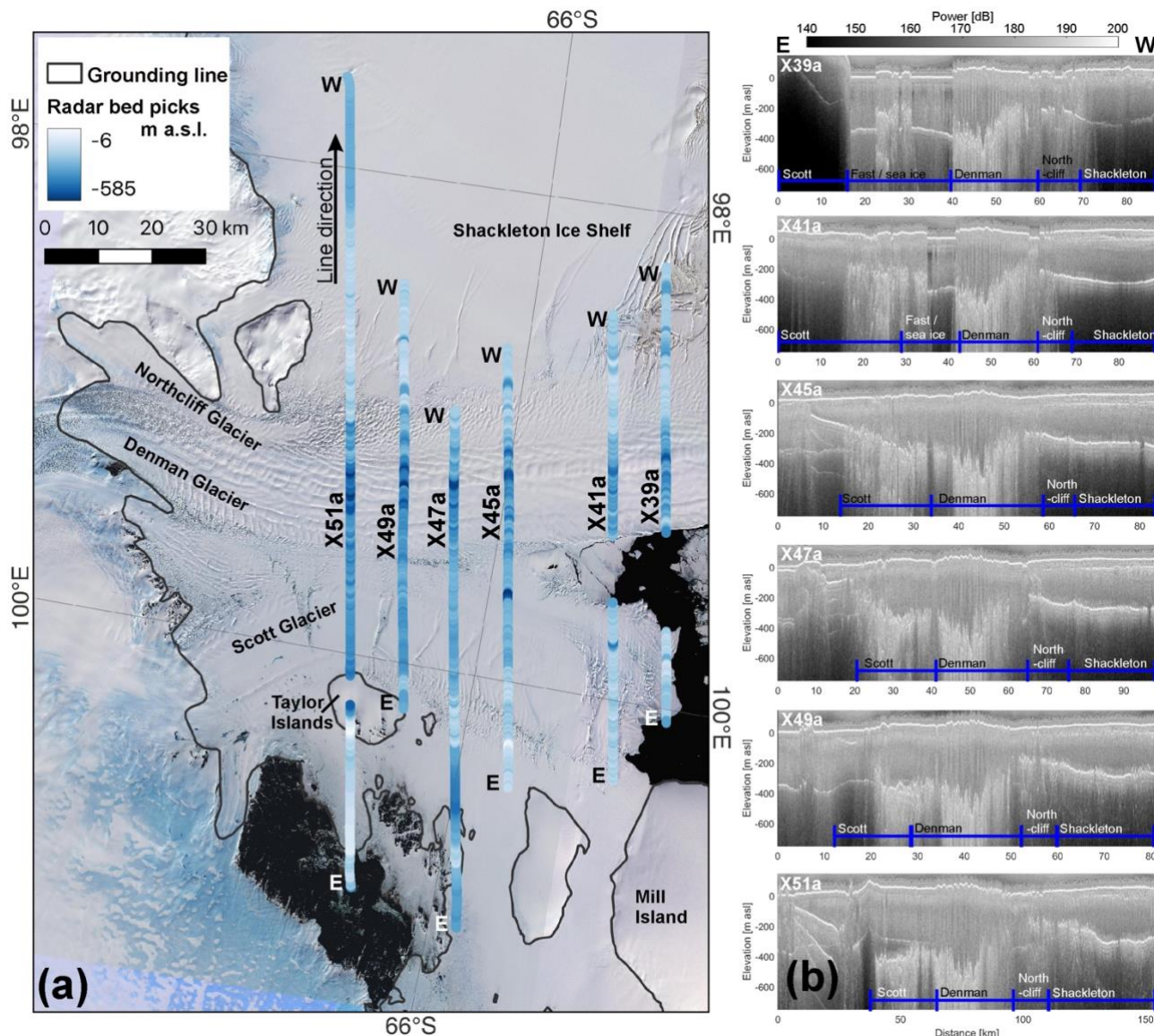
Figure 7: (a) The location and ice base below sea level of 6 ICECAP radar lines acquired in December 2016 (Background Sentinel 2A acquired 23 rd February and 1 st March 2017). (b) Annotated ICECAP radar lines (position and east-west line direction shown in a).
