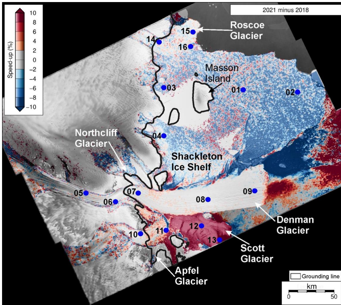
685 Figure 9: Percentage difference in mean speed between 2021 and 2018, scaled between +/- 10%, with point locations illustrating the ice speed timeseries in Figure 11.
