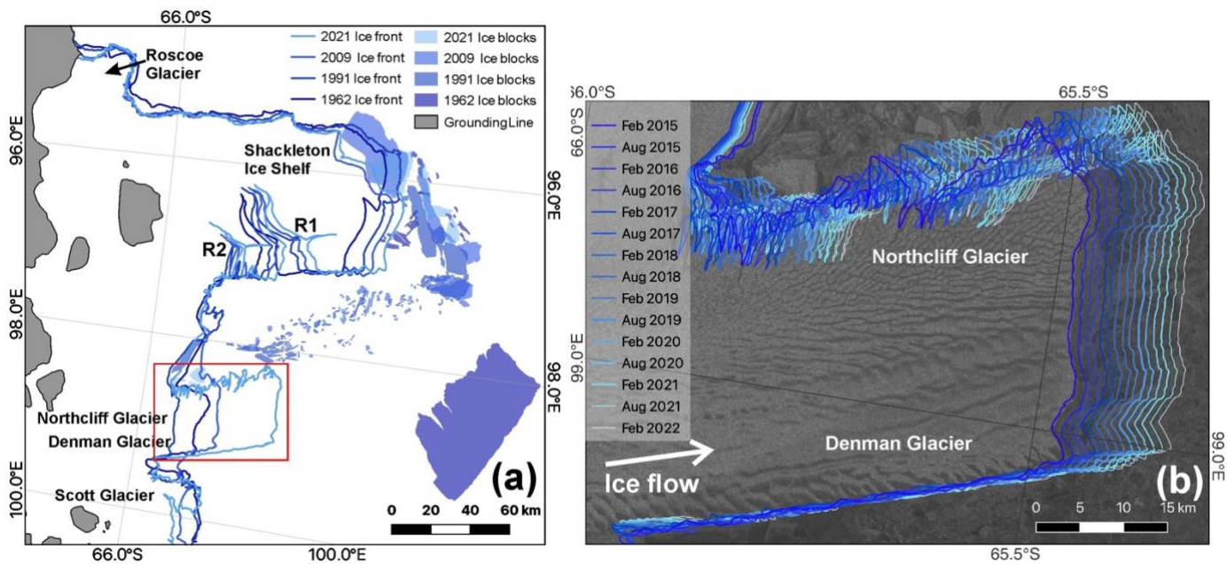
640 Figure 2: (a) Ice front positions of the Queen Mary and Knox coasts since 1962, including the large iceberg hypothesised to have calved from the Denman tongue in the 1940s. Position and blocks mapped from 16 th May 1962 – ARGON KH5, 10 th -12 th February 1991 – Landsat 5 TM, 1 st November – 28 th February 2009 – Modis MOA (Scambos et al., 2007) and 5 th – 27 th February 2021 – Sentinel 2A and 2B. The two main rift systems on the Shackleton Ice Shelf are labelled 1 and 2. (b) Denman Glacier biannual ice front position mapped in February and August from 2015 through 2022 (Background: Sentinel 1a acquired 27 th February 2015).
