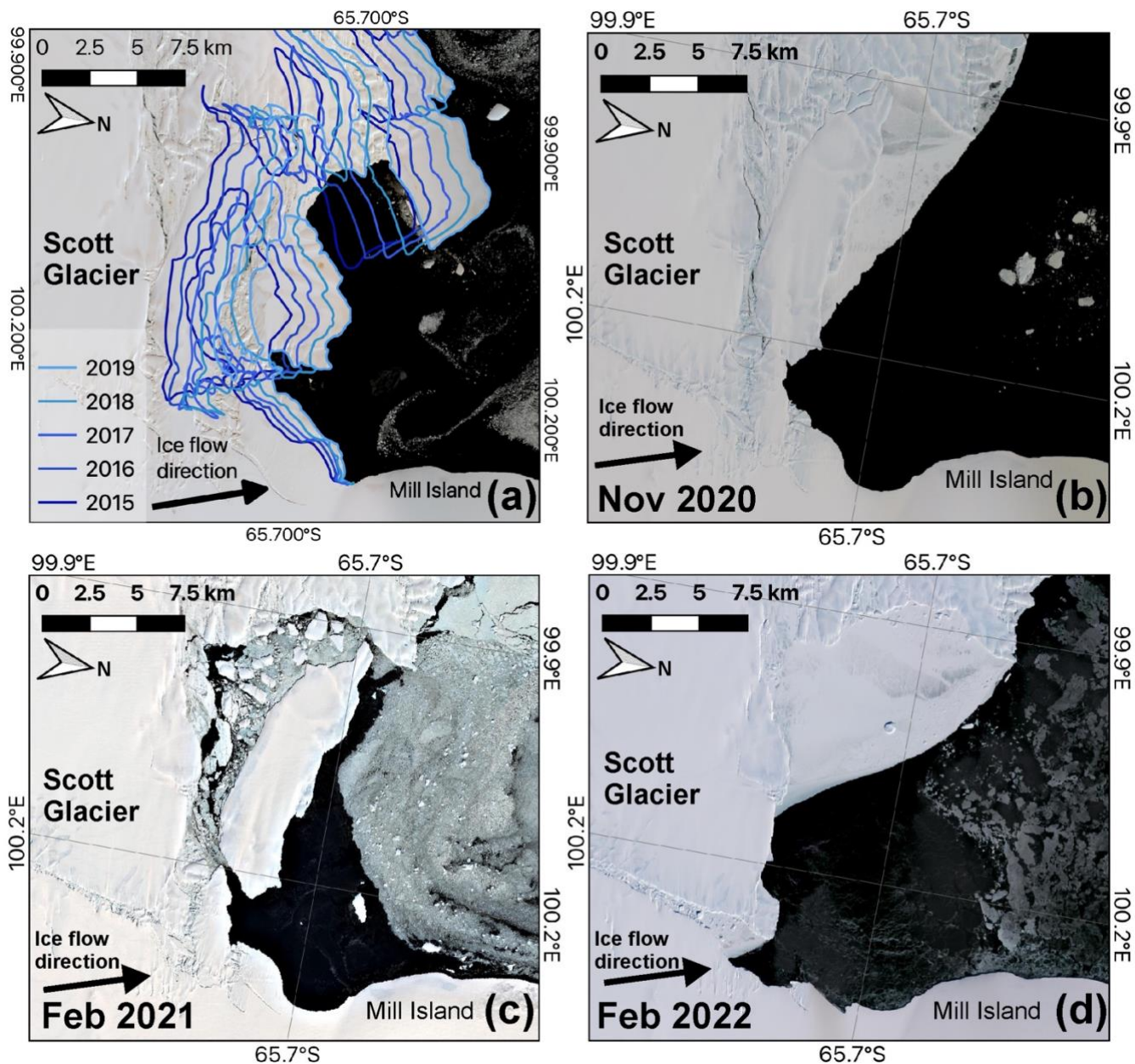
645 Figure 3: (a) Scott Glacier ice front position between 2015 and 2019 mapped from Landsat 8 OLI acquired on 16 th February 2019, 1 st February 2018, 24 th February 2016 and 7 th February 2015 and from Sentinel 2A acquired on 23 rd February 2017 (Background: Landsat 8 OLI – 16 th February 2019). (b) Scott Glacier ice front 26 th November 2020, the central portion of the front has lost some of the blocks held in place by fast ice and an area immediately to the south of Mill Island (Landsat 8 OLI), (c) Scott Glacier ice front 27 th February 2021, the fast ice has broken up and a larger block is separated (Sentinel 2B), (d) Scott Glacier ice front 21 st February 2022, (Sentinel 2B). 650
