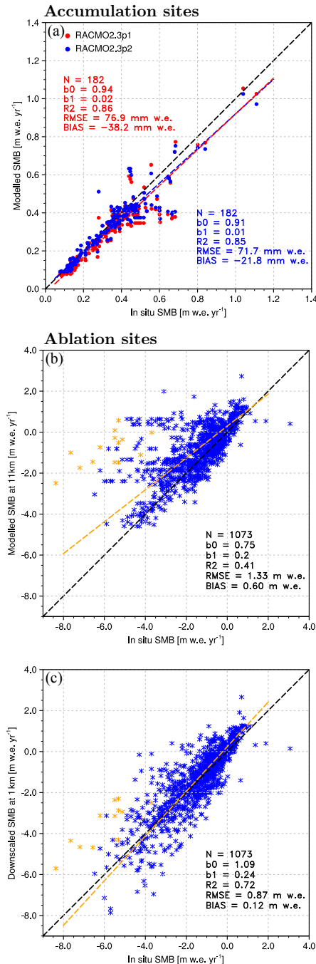
Figure 11. Comparison between (a) modelled, i.e. RACMO2.3p2 (blue) and RACMO2.3p1 (red) at 11 km, and observed SMB ( \text{m w.e. yr}^{-1} ) collected in the GrIS accumulation zone (white dots in Fig. 1). Regressions for RACMO2.3p2 (blue) and version 2.3p1 (red) are displayed as dashed lines. Comparison between SMB measurements from the GrIS ablation zone (yellow dots in Fig. 1) and (b) original RACMO2.3p2 data at 11 km, (c) downscaled product at 1 km. Orange stars correspond to measurements collected at station QAS_L at the southern tip of Greenland. Regression including all records is displayed as orange dashed line in panels (b) and (c). Main statistics including number of records ( N ), regression slope ( b_0 ) and intercept ( b_1 ), determination coefficient ( R^2 ), bias and RMSE are listed for each graph.
