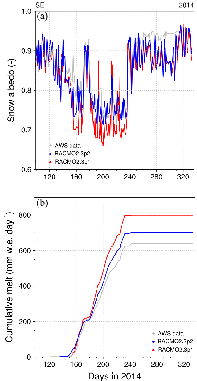
Figure 10. Time series of (a) daily snow albedo, and (b) cumulative surface melt ( \text{mm w.e. day}^{-1} ) modelled by RACMO2.3p2 (blue lines), RACMO2.3p1 (red lines) and measured (grey lines) at the south-eastern AWS ( 66^\circ \text{N} ; 33^\circ \text{W} ; 1563 \text{ m a.s.l.} ) during summer 2014.
