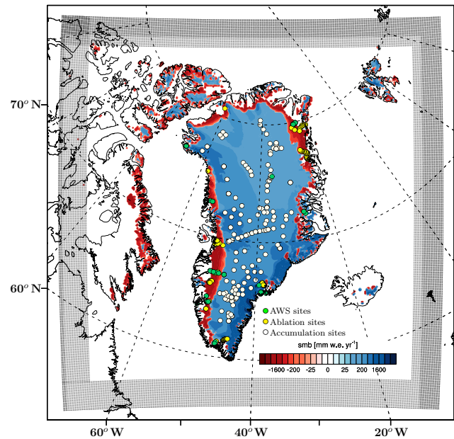
Figure 1. SMB (mm w.e. yr -1 ) modelled by RACMO2.3p2 at 11 km resolution for 2016. Black dots delineate the relaxation zone (24 grid cells) where the model is forced by ERA re-analyses. Ablation sites (213) are displayed as yellow dots, accumulation sites (182) as white dots, and AWS locations (23) are represented in green.
