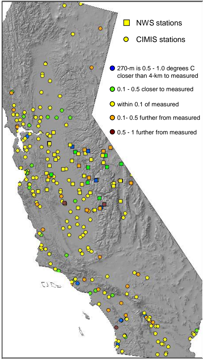
Figure 1. Station locations and error categories for the 270-m model in California.
