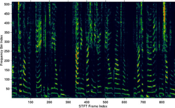
(a) spectrogram
