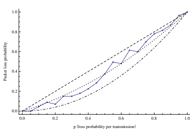
(b) Losses
