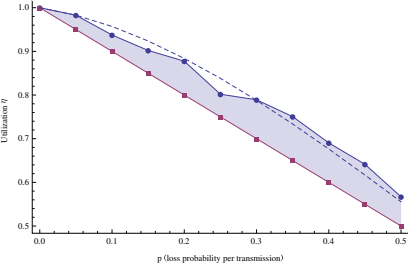
(a) Utilization
