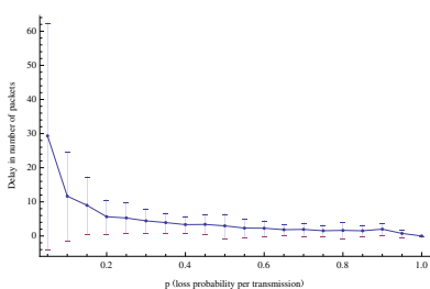
(c) Delay
