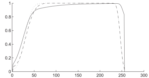
(a) \sigma_{o,j}^2 = 1
