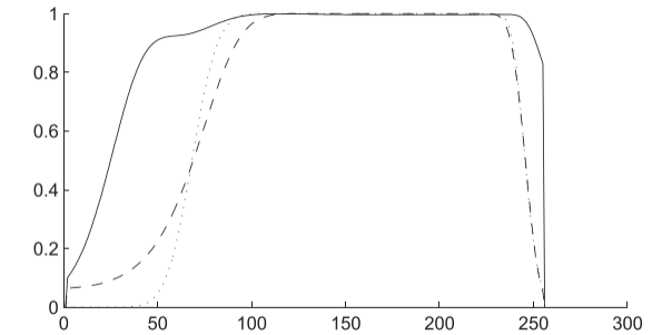
(b) \sigma_{o,j}^2 = 625
