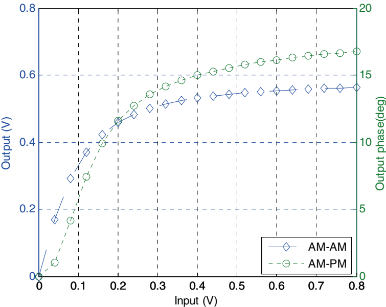
PA nonlinear
