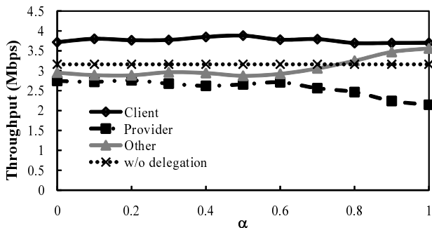
(a) \beta = 0.3
