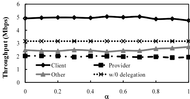
(c) \beta = 0.7
