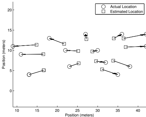
Localization with MDS and Statistical Peak Selection
