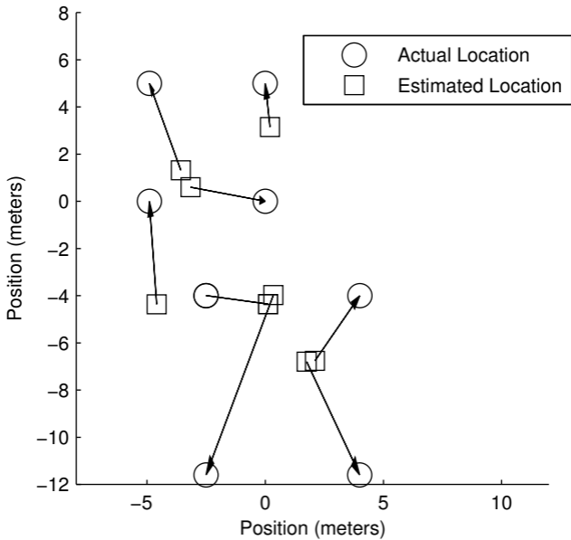
Localization with MDS and Cumulative Peak
