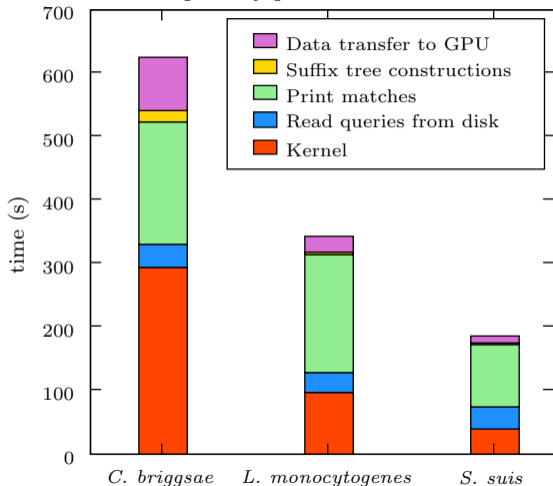
Time spent by phase in MUMmerGPU
