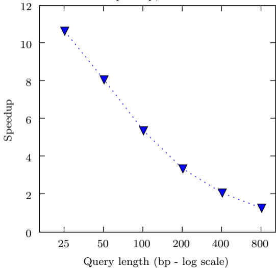
Kernel speedup, GPU vs. CPU
