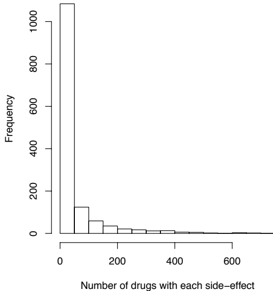
Histogram
