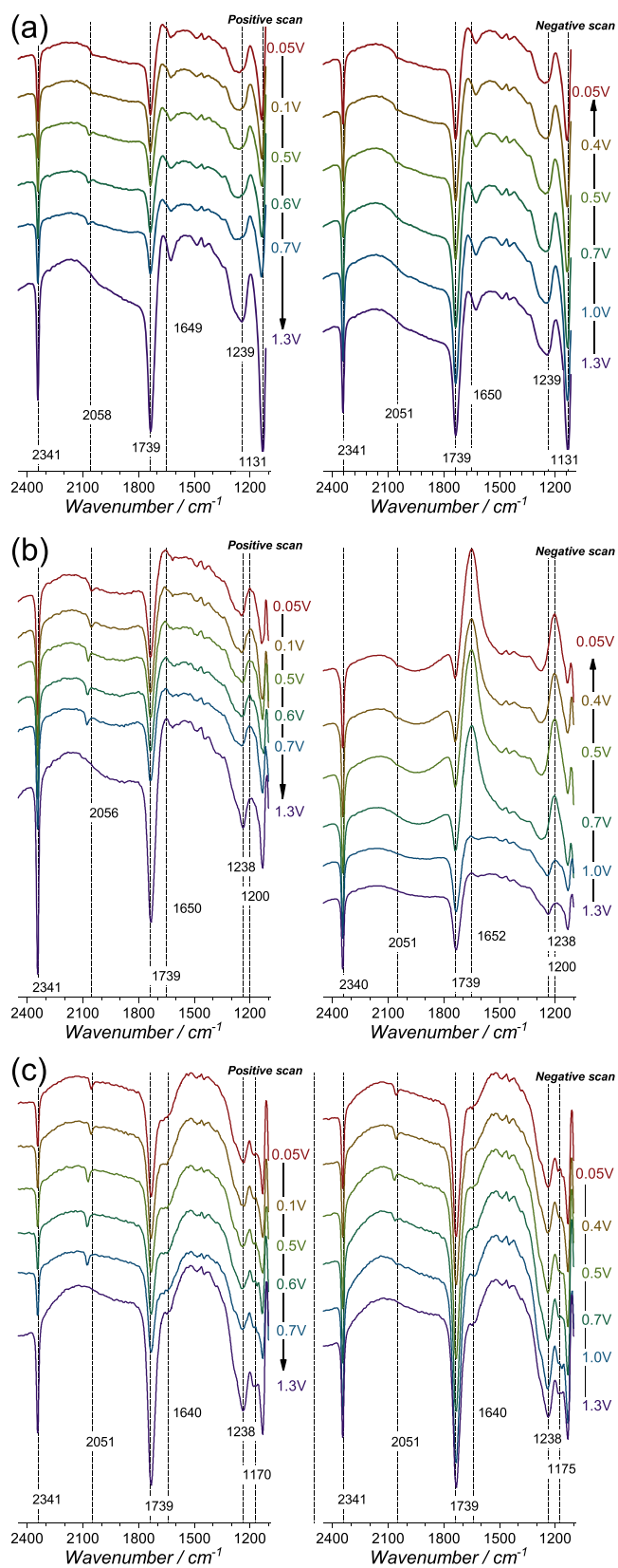
Fig. 3. Series of in situ FTIR spectra of Pt recorded (2nd scan) for consecutive potential steps cycling: positive and negative scan directions in 0.5 \text{ mol L}^{-1} glycerol + 1.0 \text{ mol L}^{-1} \text{HClO}_4 , \text{H}_2\text{SO}_4 and \text{H}_3\text{PO}_4 . Sample spectra were collected at the indicated potentials.
