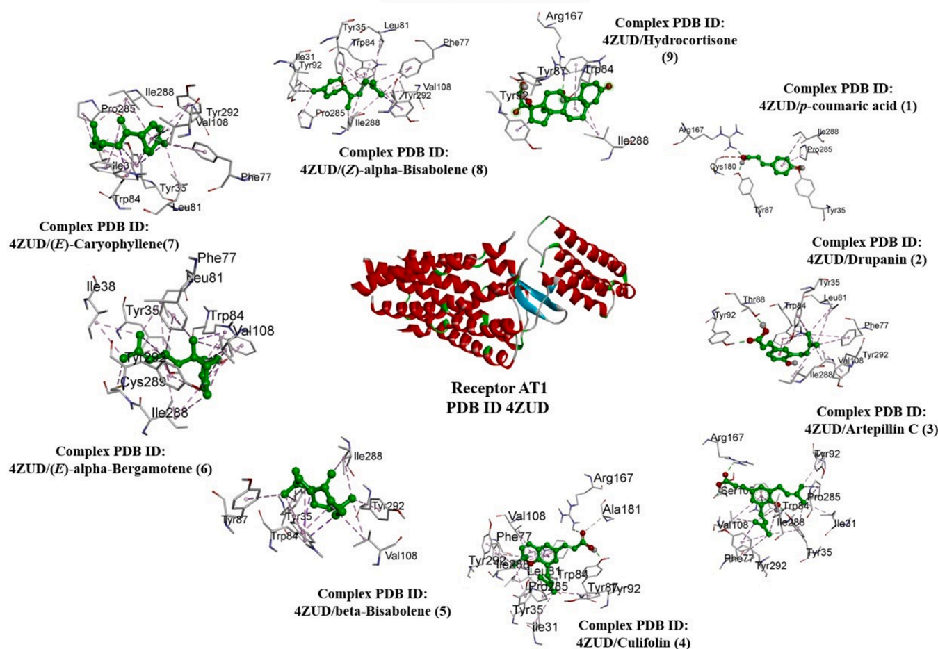
Fig. 7. : General bindings about the main compounds founded in PRO, COR, and H with the Receptor AT 1 (AT 1 R) in Protein Data Bank (PDB) ID 4ZUD. Complexes: (1) Coumaric acid; (2) Drupanin; (3) Artepillin C; and (4) Culiifolin; (5) \beta -bisabolene; (6) ( E )- \alpha -bergamotene; (7) ( E )-caryophyllene; (8) ( Z )- \alpha -bisabolene; and (9) Hydrocortisone.
