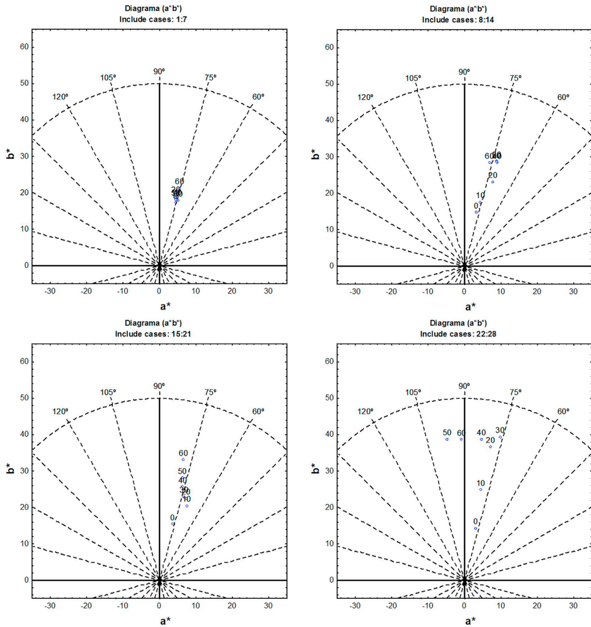
Fig. 4. CIELAB color space (a*b* - plan) for sugarcane juice treated by electrocoagulation. (a) 35 V essay; (b) 45 V essay; (c) 55 V essay; (d) 65 V essay.
