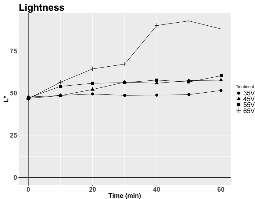
Fig. 2. Evolution of lightness parameter of CIELAB (L*) for each treatment.
