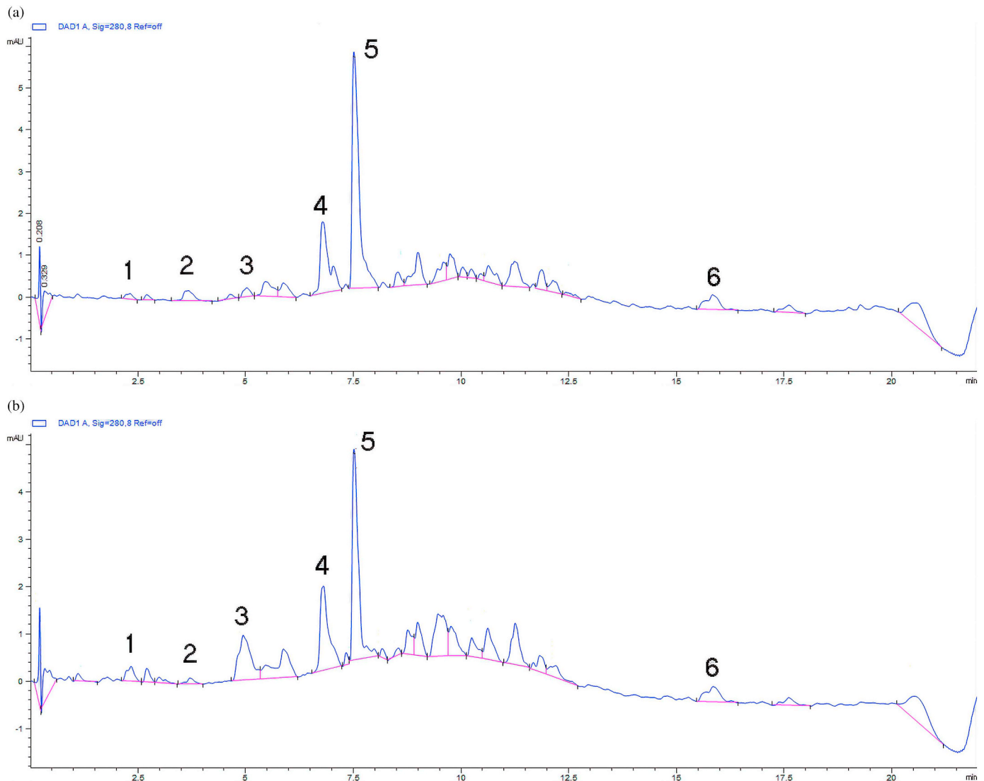
Fig. A1. (a) Chromatogram of untreated juice before the electrocoagulation process. (b) Chromatogram of sugarcane juice treated electrocoagulation (65 V essay – 60 min). In both figures: (1) gallic acid, (2) p-Hydroxibenzoic acid, (3) vanillic acid, (4) syringic acid, (5) p-Coumaric acid, (6) naringenin.
