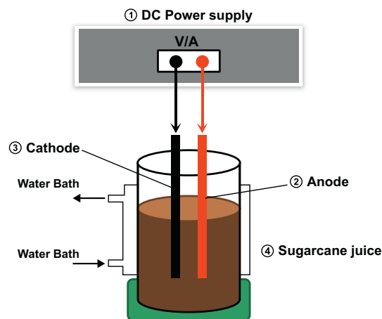
Fig. 1. Electrocoagulation glass reactor.
