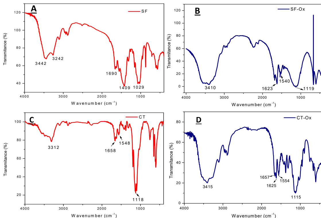
Figure 4. FTIR spectra of silk-fibroin (A) and silk-fibroin-Oxone® (B); chitin (C) and chitin-Oxone® (D).
