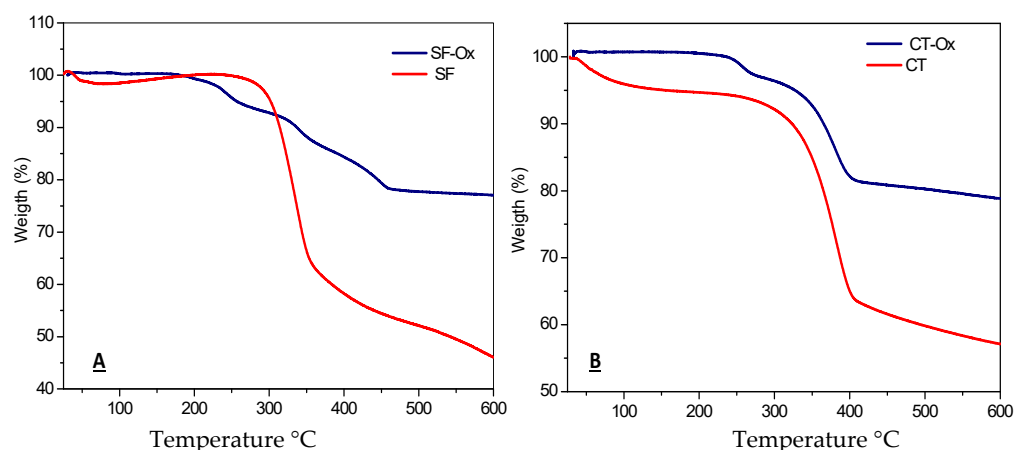
Figure 5. Thermogravimetric analysis of the biopolymers SF-Ox and SF (A); CT-Ox and CT-Ox (B).
