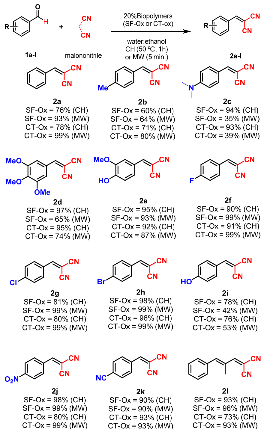
Figure 2. Knoevenagel condensation synthesis using aromatic aldehyde derivatives, malononitrile and immobilized biopolymers with Oxone ® as catalysts under conventional heating (CH) or with microwave irradiation (MW) as a heating source.
