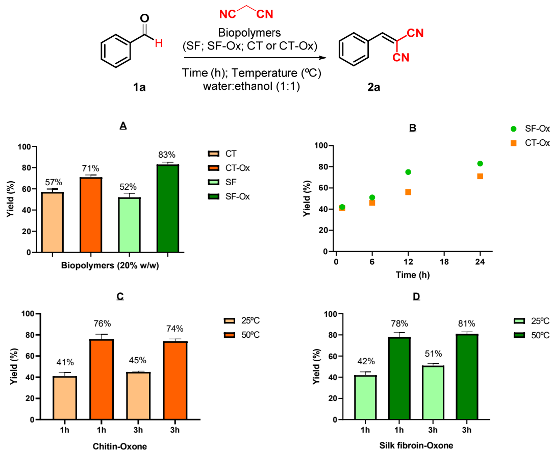
Figure 1. Optimization of Knoevenagel condensation reaction using aldehyde 1a (2 mmol) and malononitrile (2.5 mmol) with and without biopolymers (20% w/w ) as catalysts. (A) Screening of biopolymers (rt and 24 h); (B) effect of time [1, 3, 6, 12 and 24 h (r.t.)] in presence of CT-Ox and SF-Ox; (C) effect of temperature (25 or 50 °C for 1 or 3 h) with CT-Ox; (D) effect of temperature (25 or 50 °C at 1 or 3 h) with SF-Ox.
