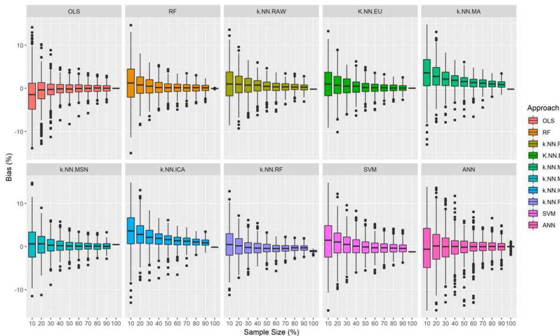
Figure 5. Modeling methods’ performance in terms of bias derived from the 500 bootstrapping simulations for each sample size.
