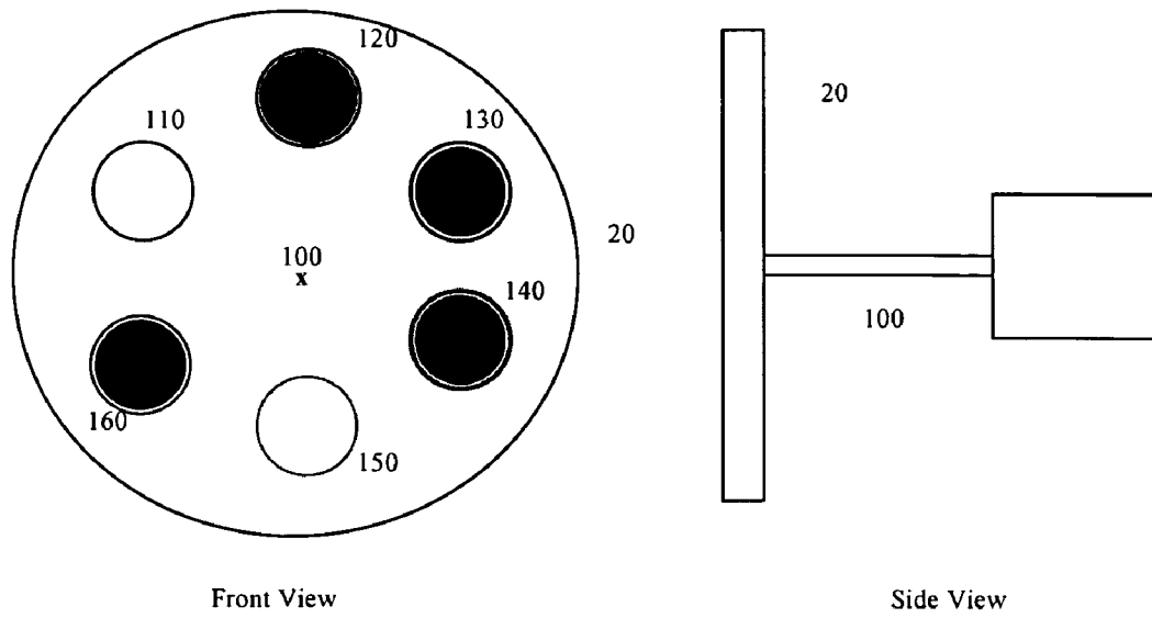
FIG.2 Rotating Disk with filter Set.
