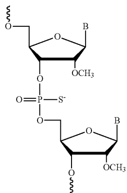
2'O-Methyl PS
