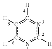
Pyrimidine
