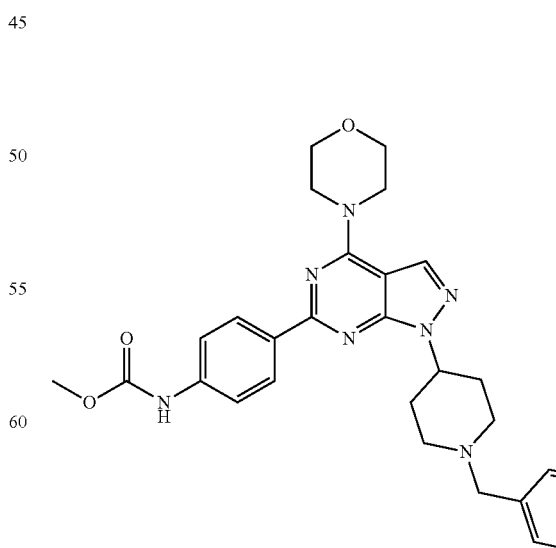
WYE 687
