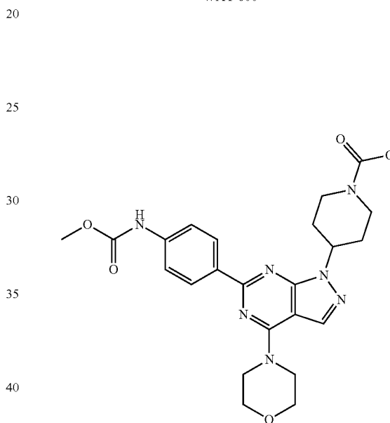
WYE-354
