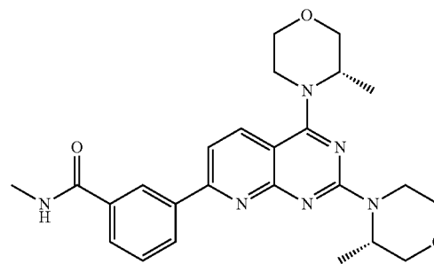
AZD 2014 (vistusertib)
