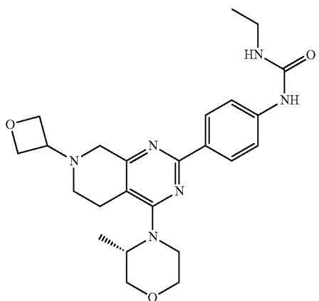
GDC-0349
