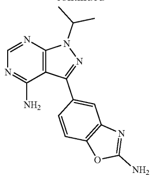
INK 128
