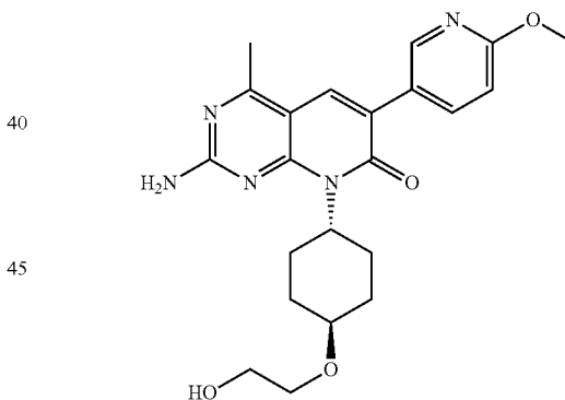
PF-04691502
