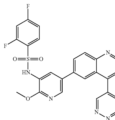
omipalisib
