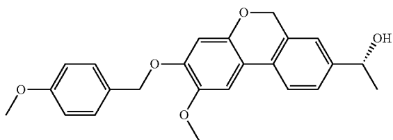
palomid 529
