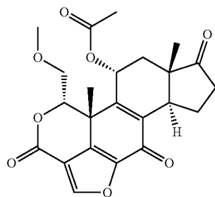
wortmannin
