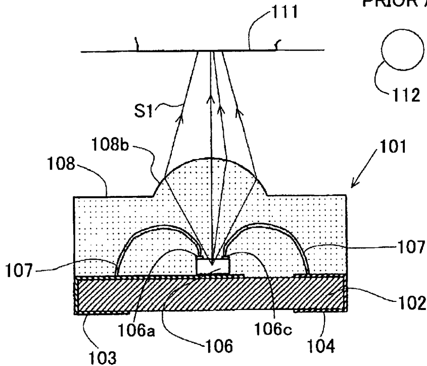
FIG. 8 PRIOR ART
