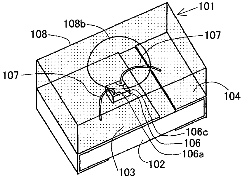
FIG. 8 PRIOR ART
