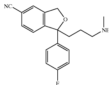
desmethyl citalopram
