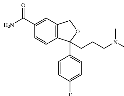
5-carboximide citalopram
