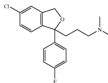
5-Br/Cl-citalopram
