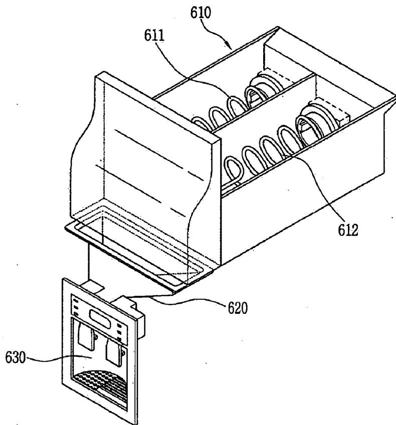
Figure 6 Prior Art
