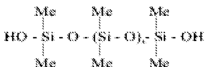
Dimethiconol
