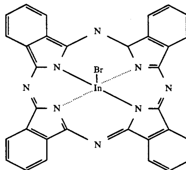
bromoindium phthalocyanine ("BrInPc")
