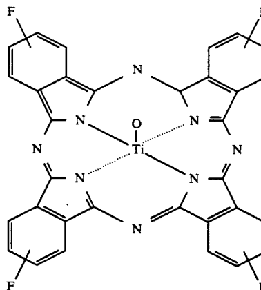
tetrafluoro- phthalocyanine ("TiOPcF4")
