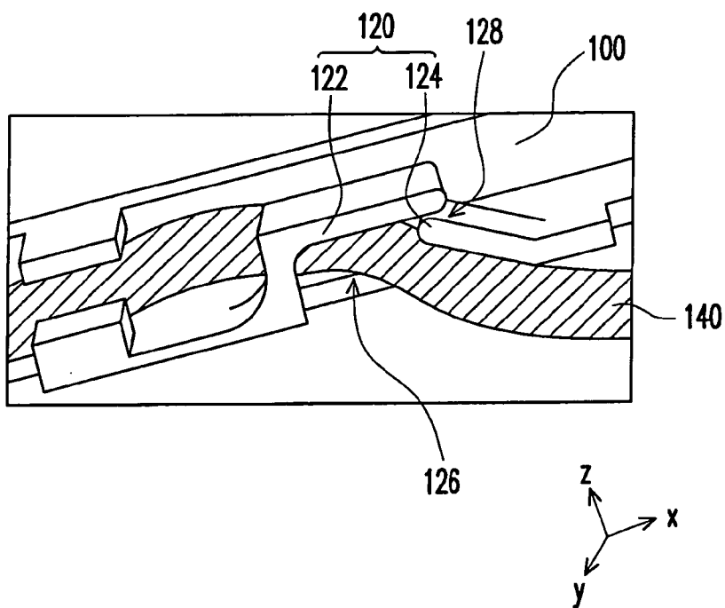
FIG. 1 (PRIOR ART)
