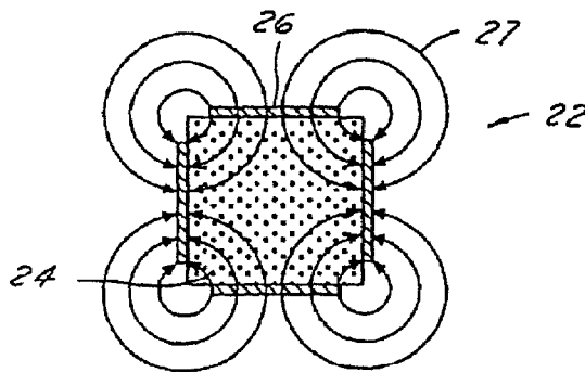
CROSS-SECTION OF TUNING FORK TINE
